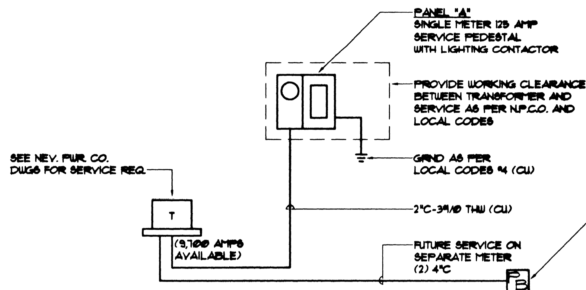
1 POWER RISER DIAGRAM E-2 SCALE: NONE
