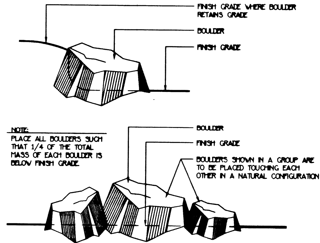
E BOULDER PLACEMENT DETAIL
