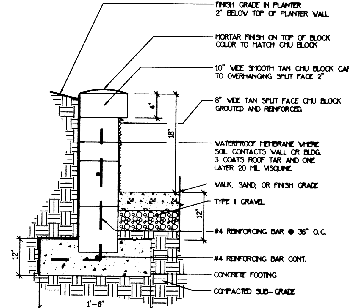
I PLANTER WALL DETAIL
