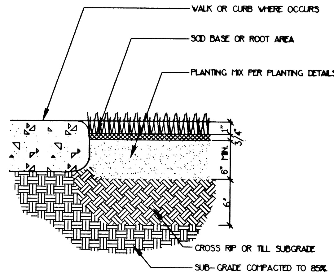
D SOD PLANTING DETAIL
