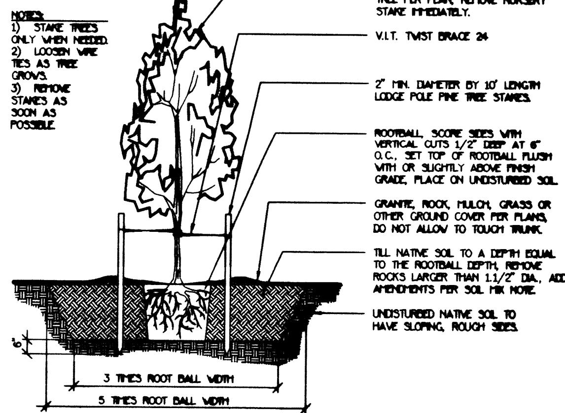
A TREE PLANTING DETAIL
