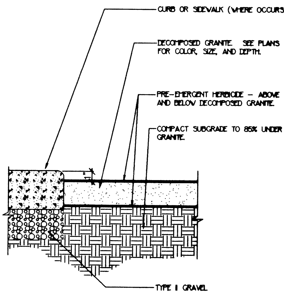
F DECOMPOSED GRANITE DETAIL
