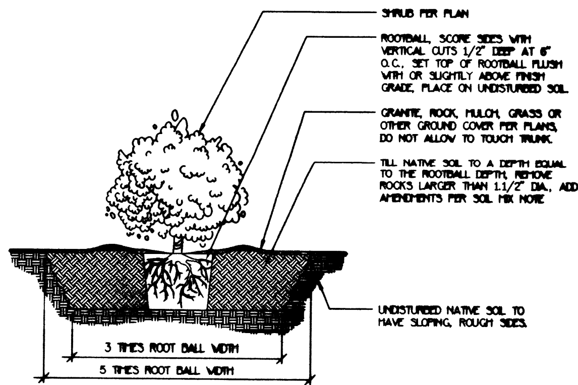
B SHRUB PLANTING DETAIL
