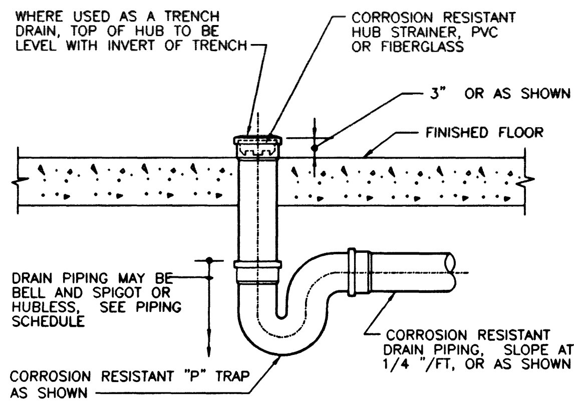
CORROSION RESISTANT HUB DRAIN REV 082796 M-315
