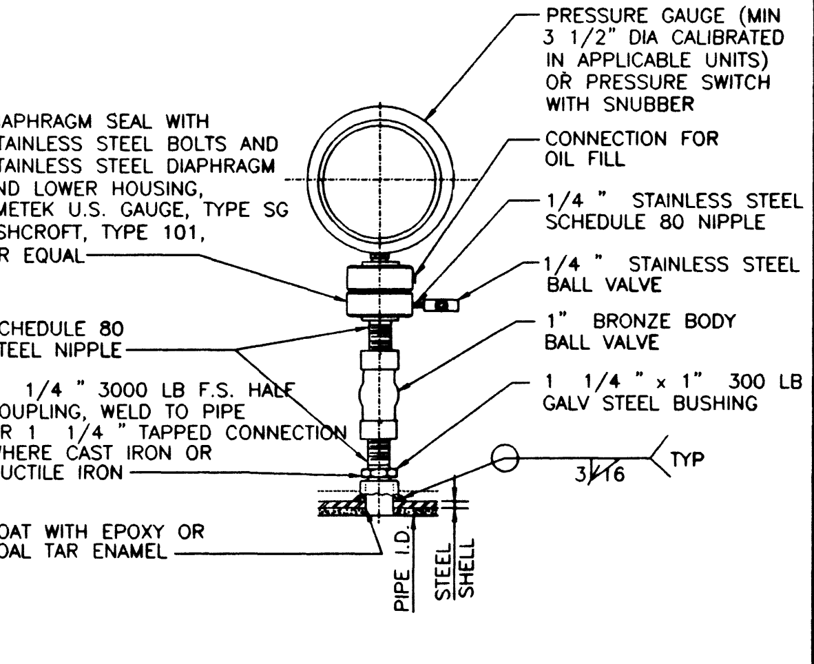
PRESSURE GAUGE AND PRESSURE SWITCH WITH DIAPHRAGM SEAL REV 082796 M-608
