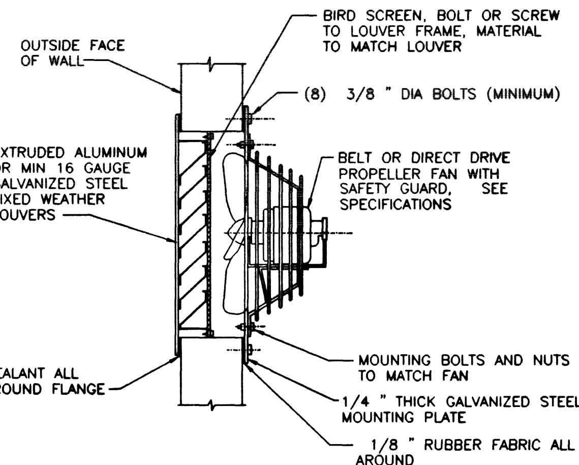
FAN WITH FIXED LOUVER REV 082796 M-505
