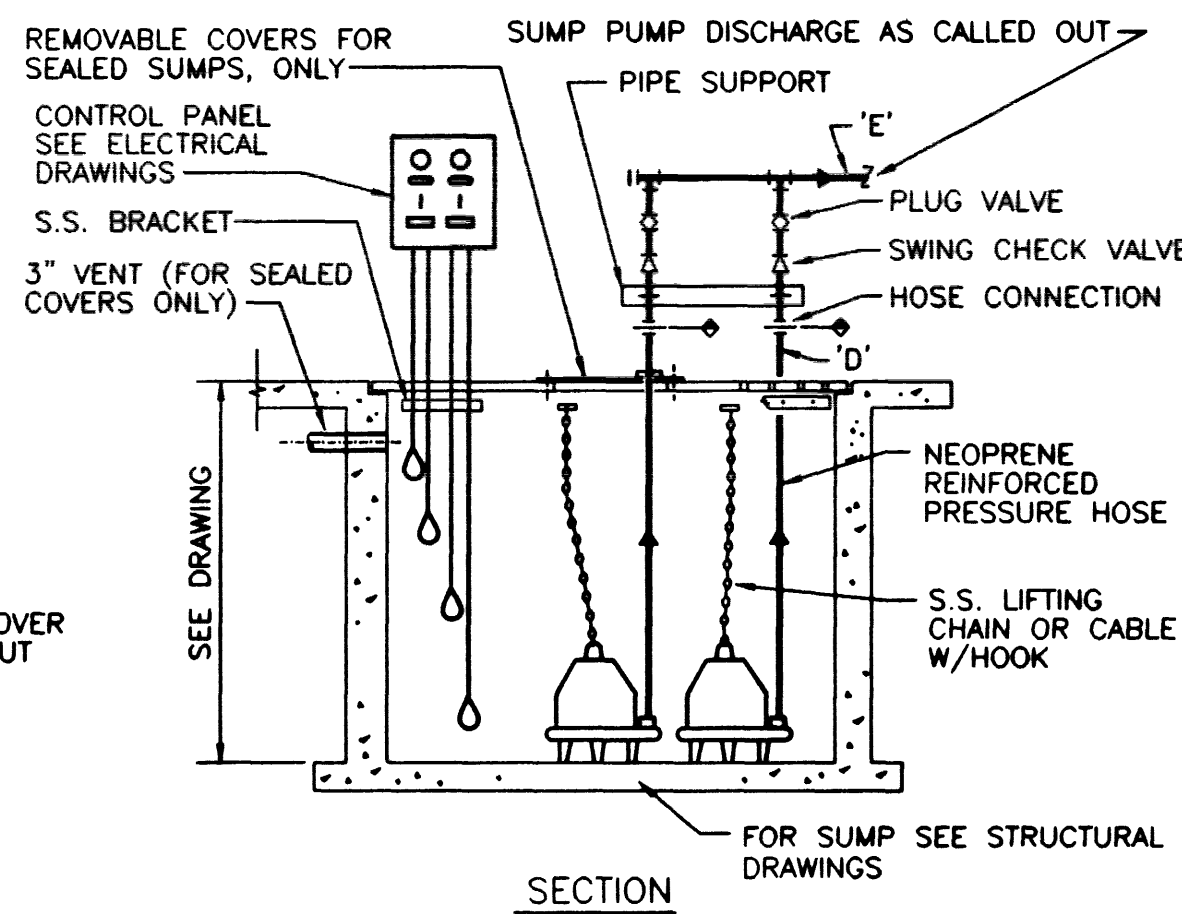
DRAINAGE SUMP WITH DUPLEX PUMPS REV 082796 M-316
