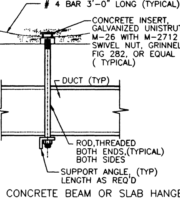
CONCRETE BEAM OR SLAB HANGER
