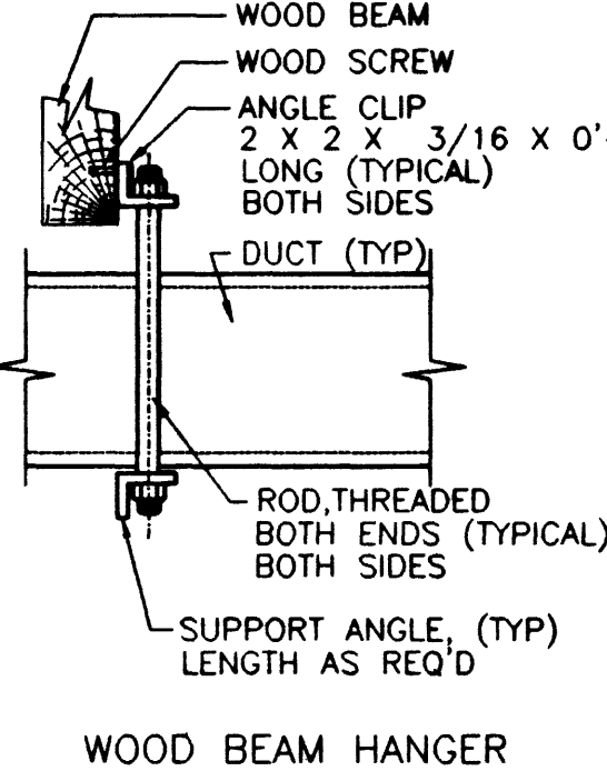
WOOD BEAM HANGER
