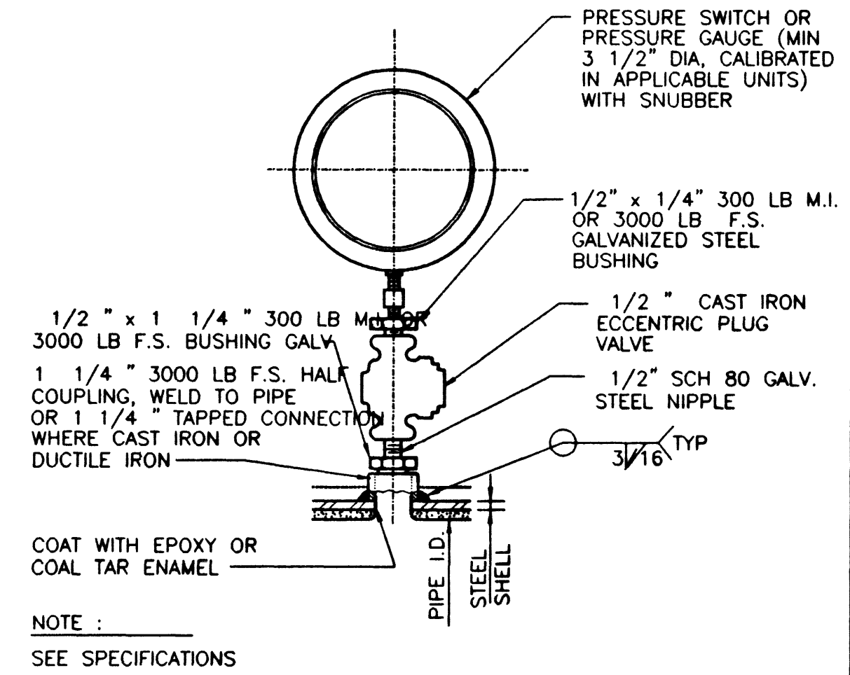
PRESSURE GAUGE OR PRESSURE SWITCH REV 082796 M-606
