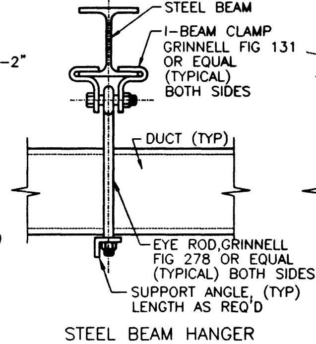
STEEL BEAM HANGER
