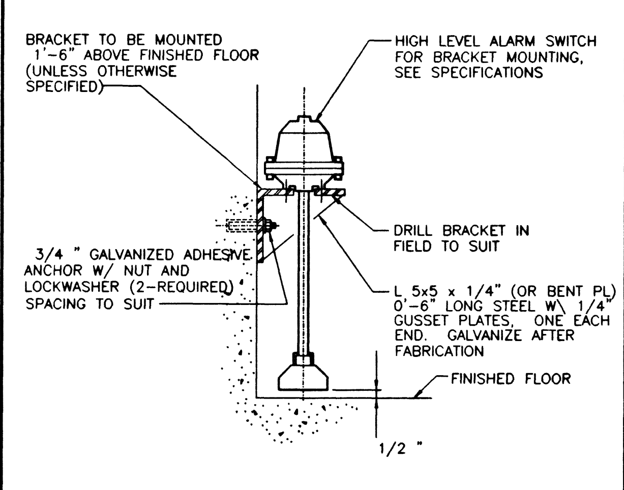
FLOOD ALARM SWITCH REV 082796 M-607
