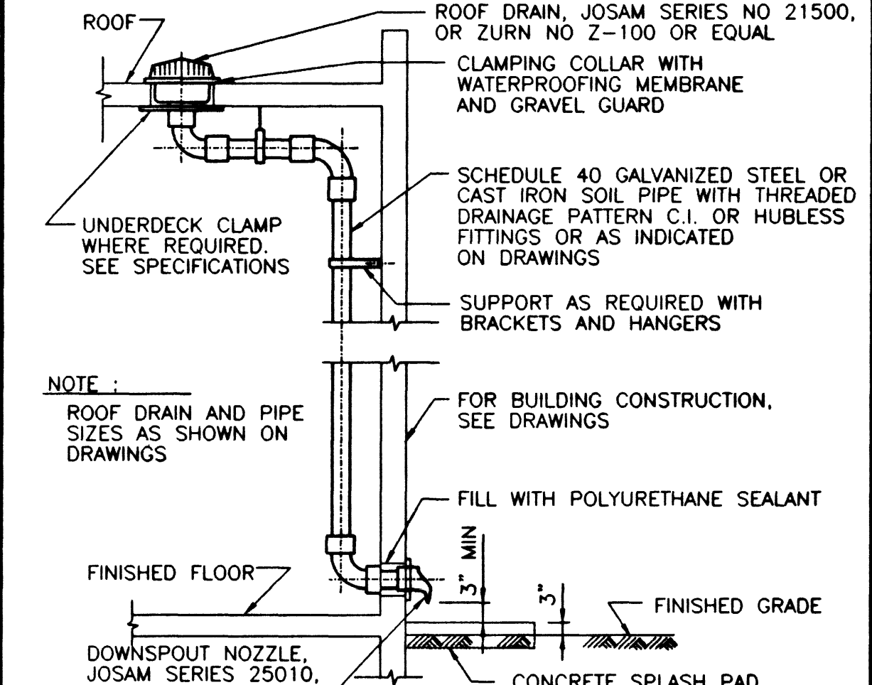
RAINWATER LEADER REV. 100796 M-314
