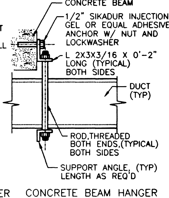
CONCRETE BEAM HANGER
