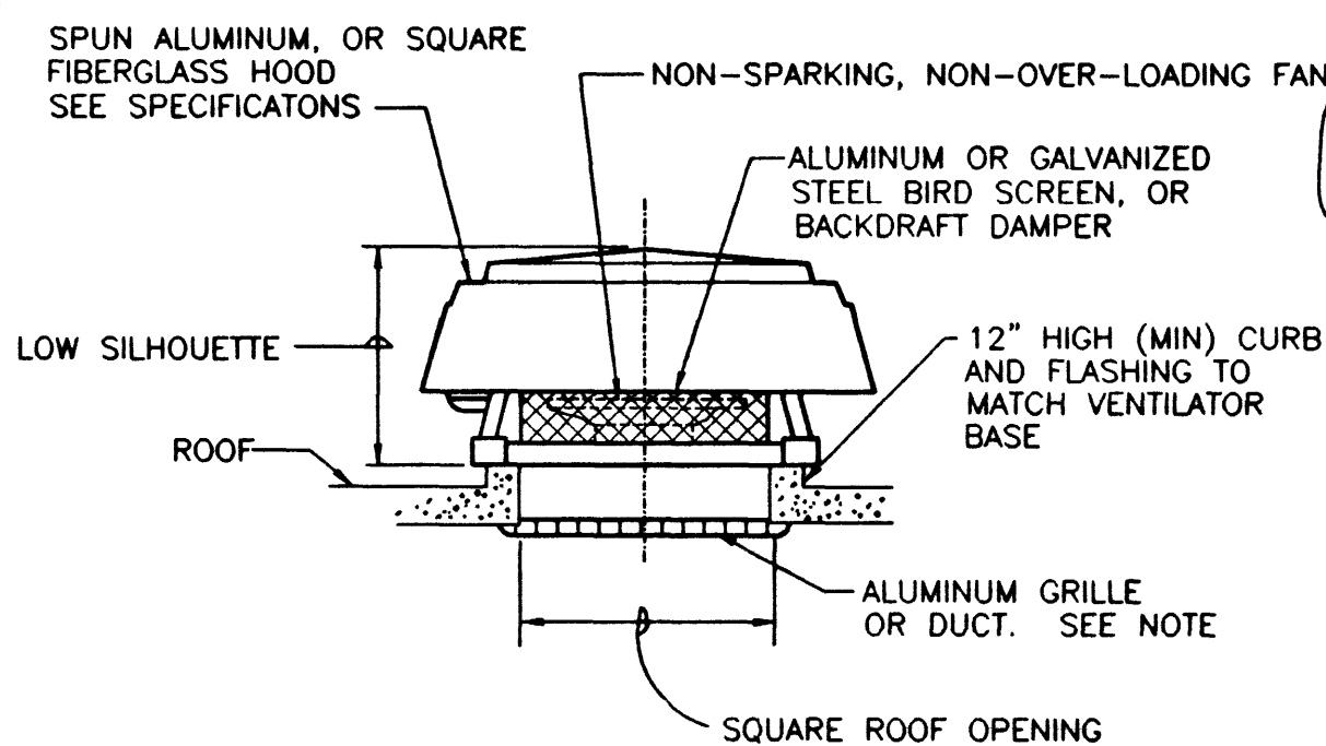
POWER ROOF VENTILATOR REV 082796 M-515
