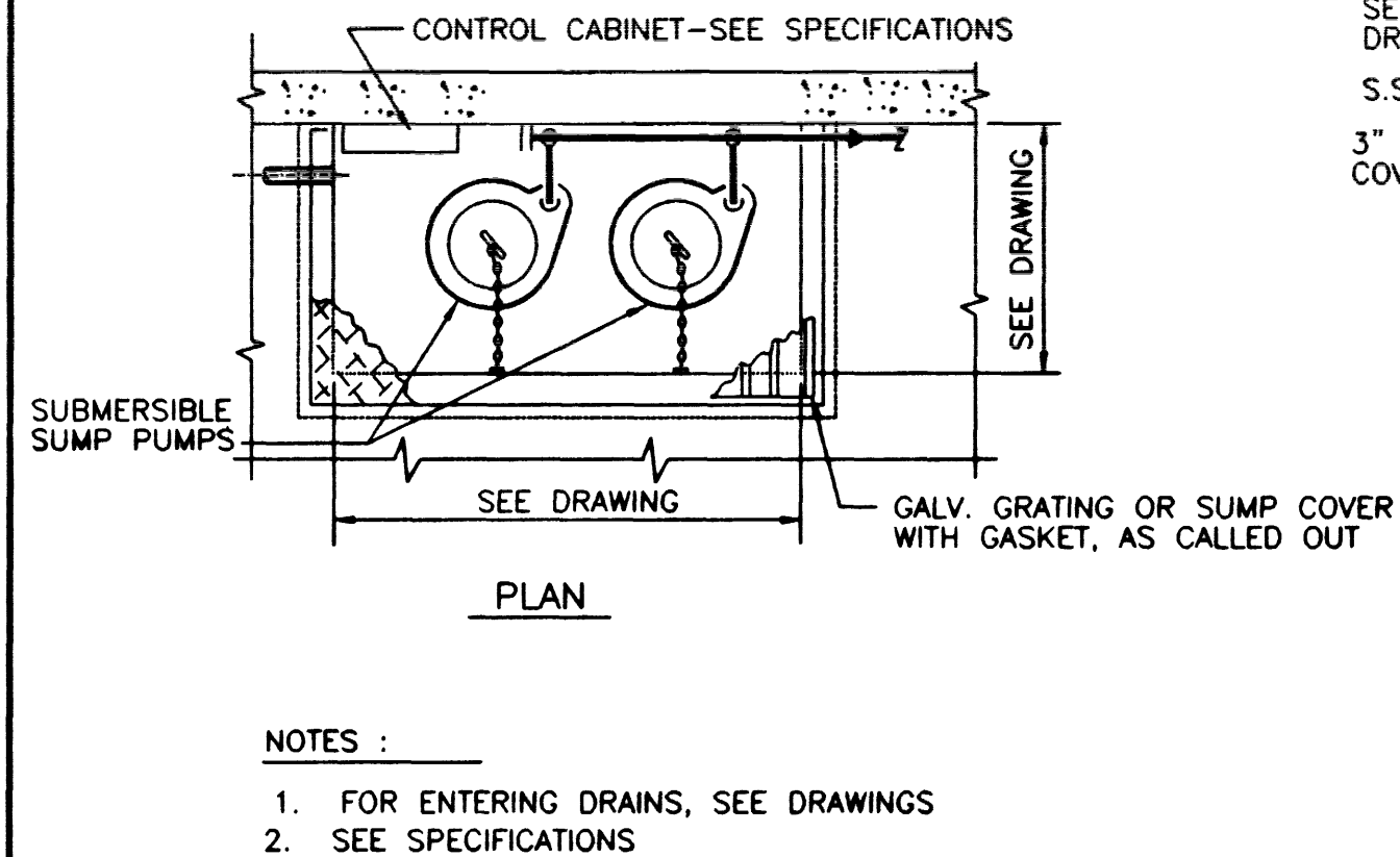
DRAINAGE SUMP WITH DUPLEX PUMPS REV 082796 M-316
