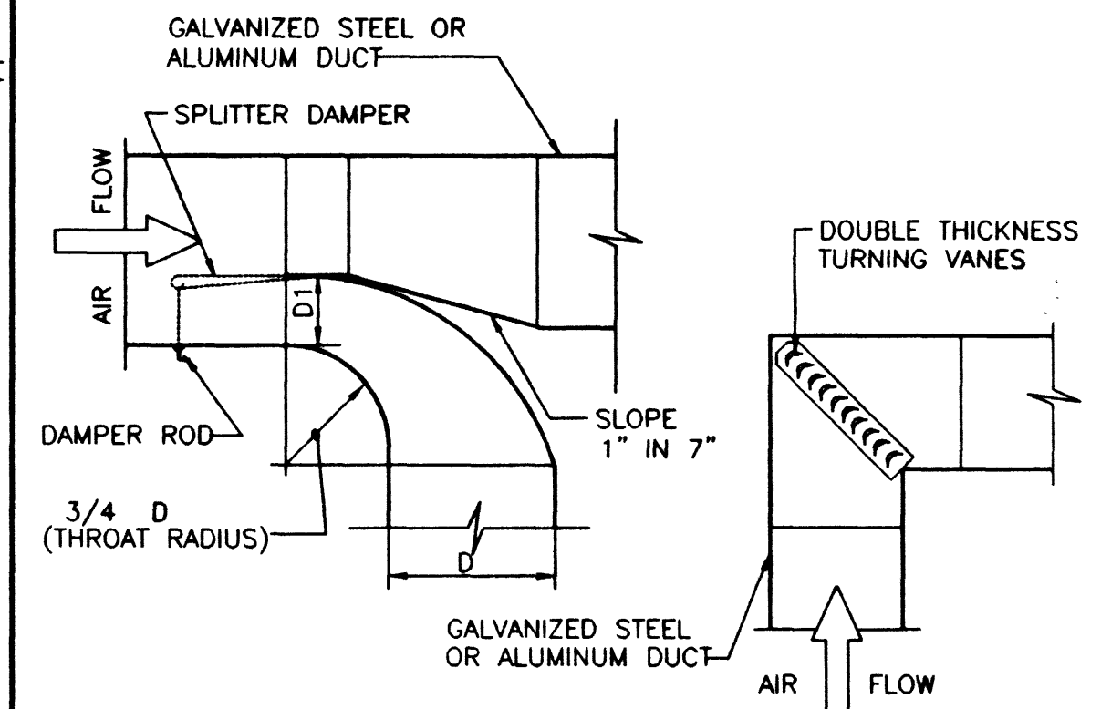
TYPICAL SUPPLY AIR DUCT BRANCH NOTE: SEE SPECIFICATIONS TYPICAL SHARP TURN WITH TURNING VANES
