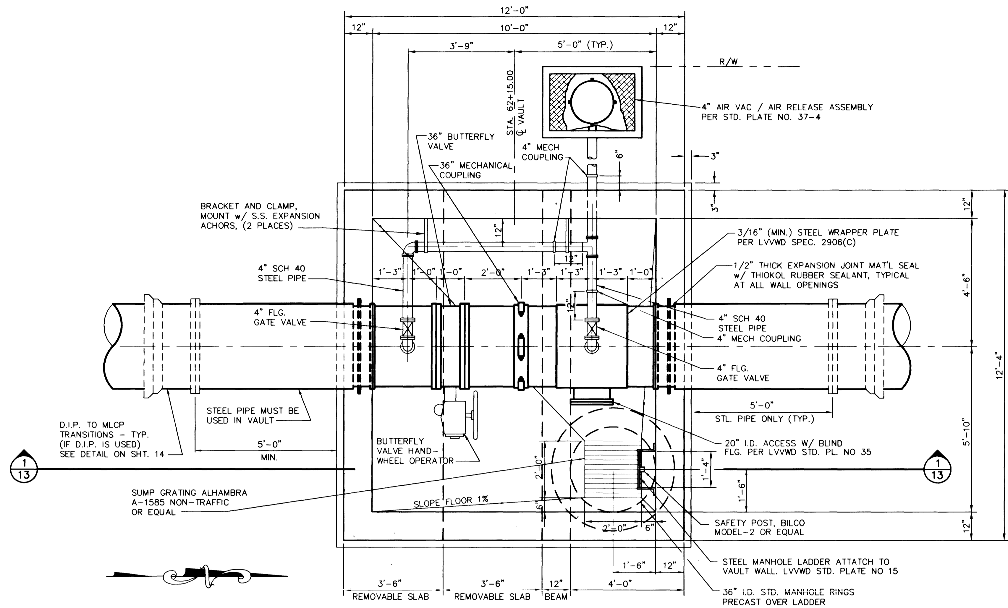
VALVE VAULT #2 PLAN SCALE: 1/2"=1'-0"
