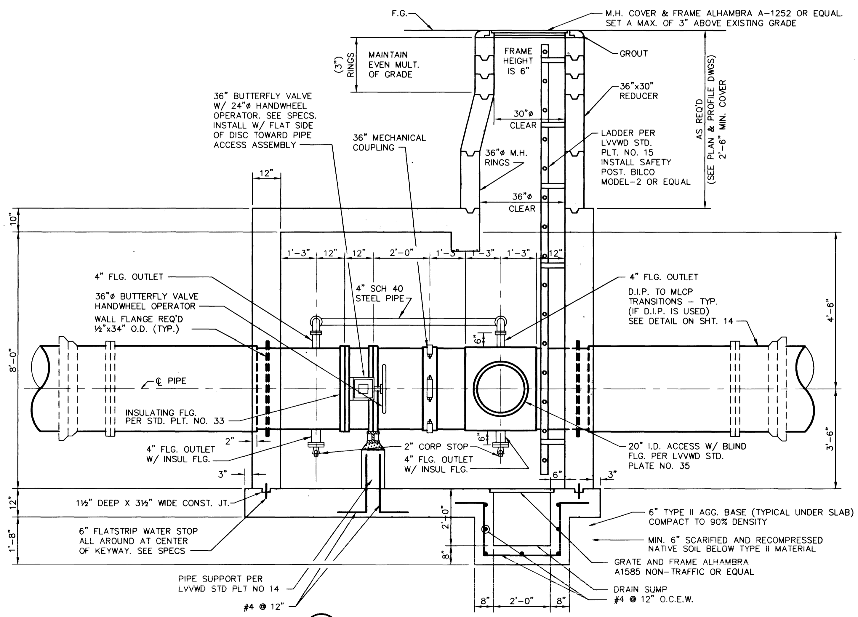
VALVE VAULT #2 SECTION SCALE: 1/2"=1'-0"
