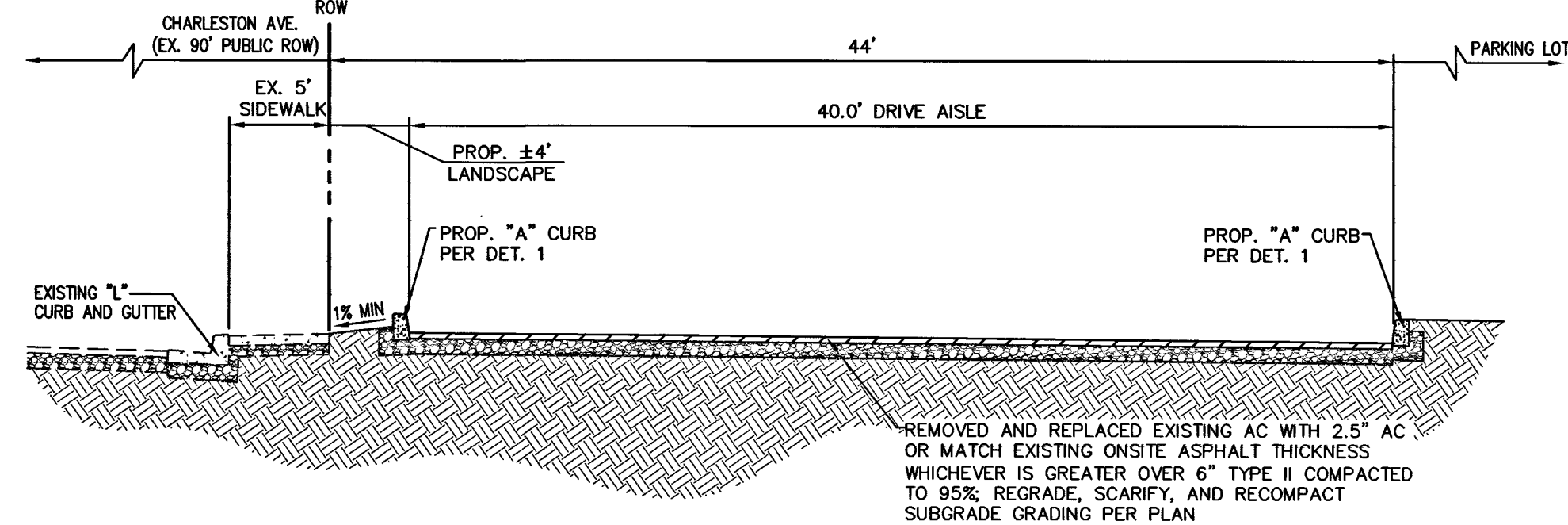
B SECTION 'B' ON-SITE SECTION NTS
