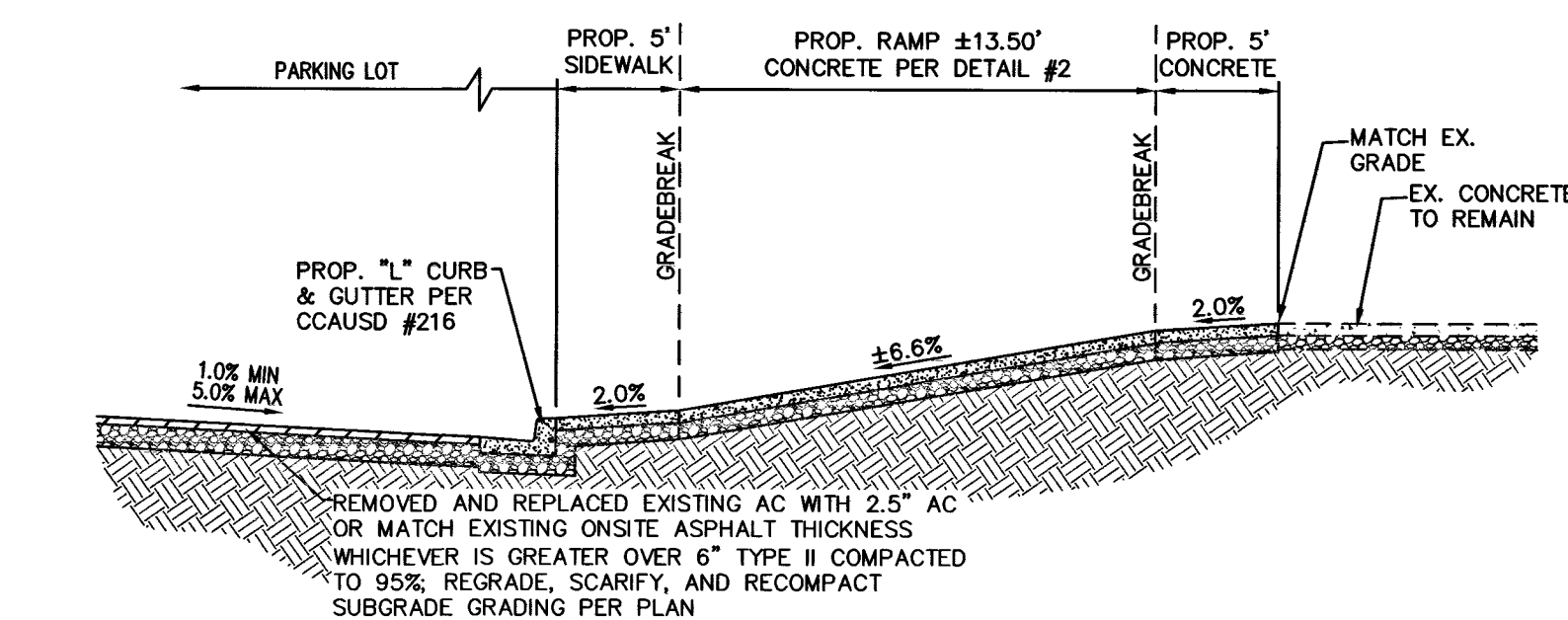
E SECTION 'E' ON-SITE SECTION NTS
