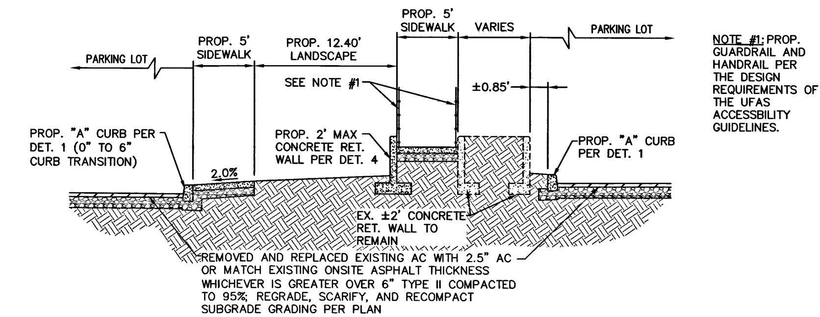
D SECTION 'D' ON-SITE SECTION NTS
