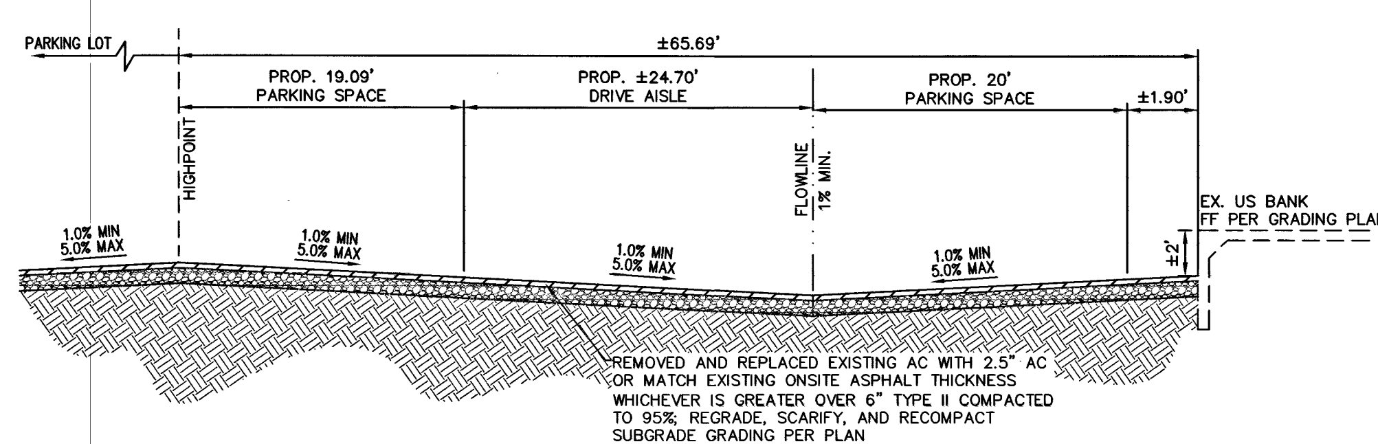
F SECTION 'F' ON-SITE SECTION NTS
