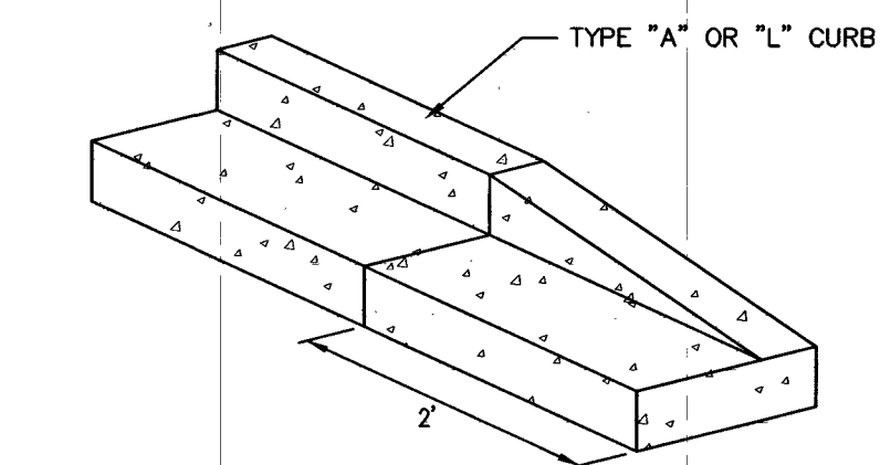
3 2' CURB TAPARED END DETAIL NTS
