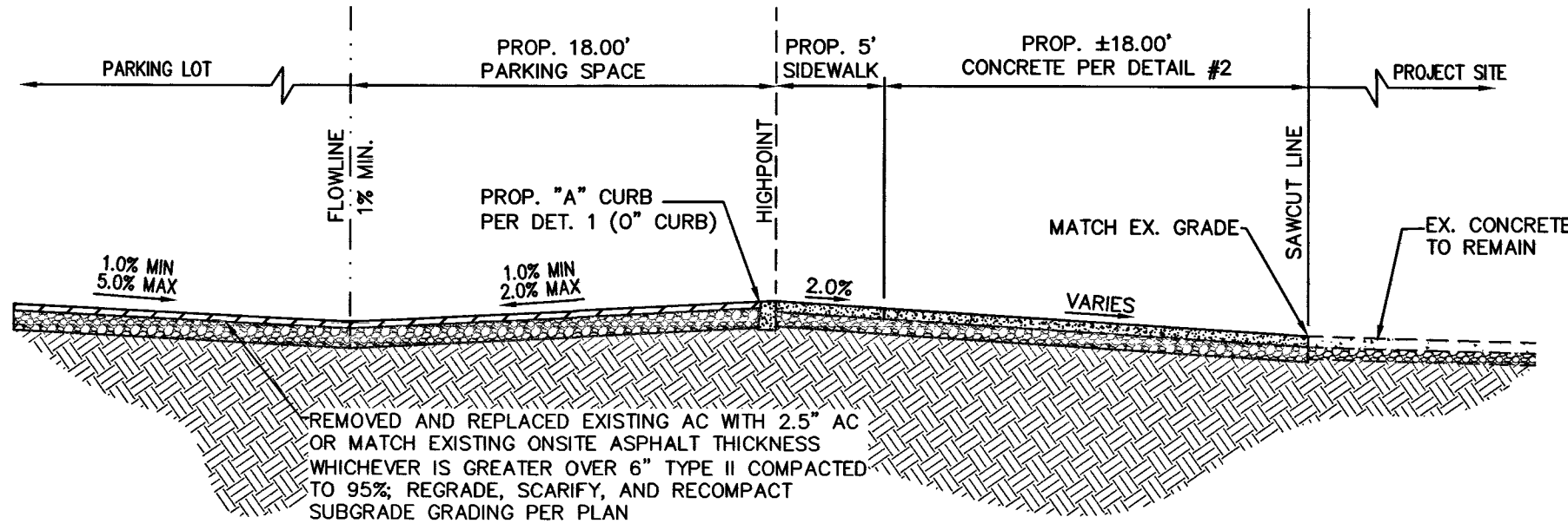
C SECTION 'C' ON-SITE SECTION NTS
