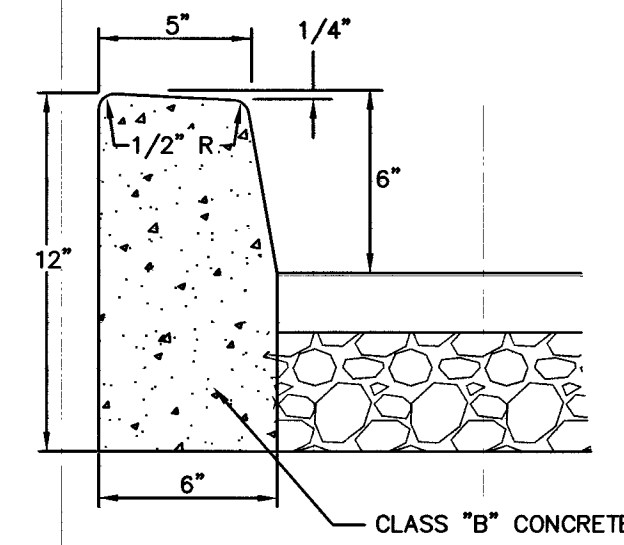
1 TYPE 'A' CURB SECTION NTS
