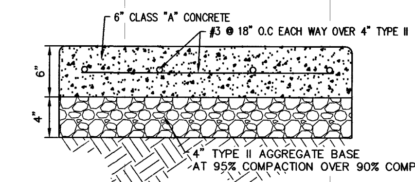
5 TRAFFIC RATED CONCRETE DETAIL (REINFORCED) NTS
