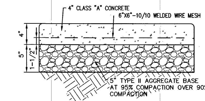
2 REINFORCED CONCRETE DETAIL NTS
