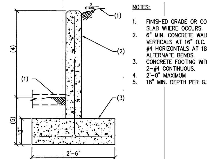
4 2' MAX CONC. RET. WALL DETAIL (CAST-IN-PLACE CONCRETE WALLS) NTS
