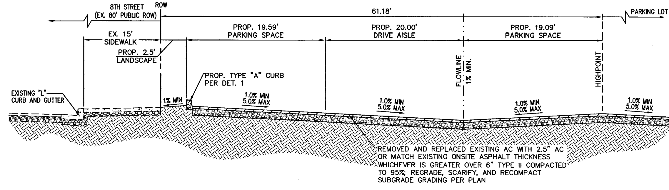
A SECTION 'A' ON-SITE SECTION NTS
