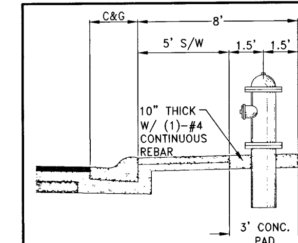
PUBLIC FIRE HYDRANT INSTALLATION WITH SIDEWALK PER UDACS PLATE NO. 40
