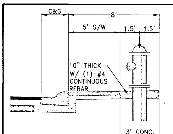
PUBLIC FIRE HYDRANT INSTALLATION WITH SIDEWALK PER UDACS PLATE NO. 40
