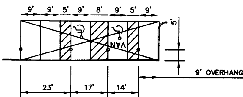
TYPICAL HC COVERED PARKING SEE SHEET 18 FOR CURB AND LINE TABLE
