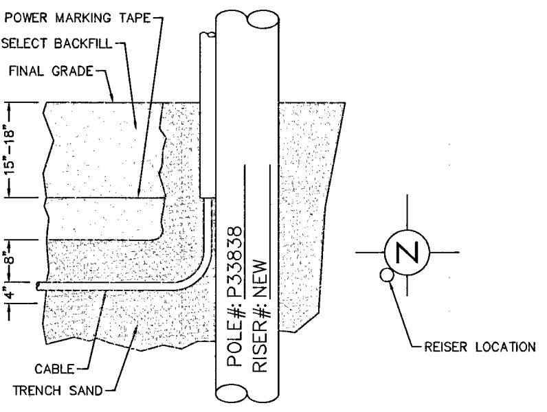
RISER DETAIL DIRECT BURIED CABLE & CABLE IN CONDUIT PER NVE U.G. STD. RR-1 (TYP.)
