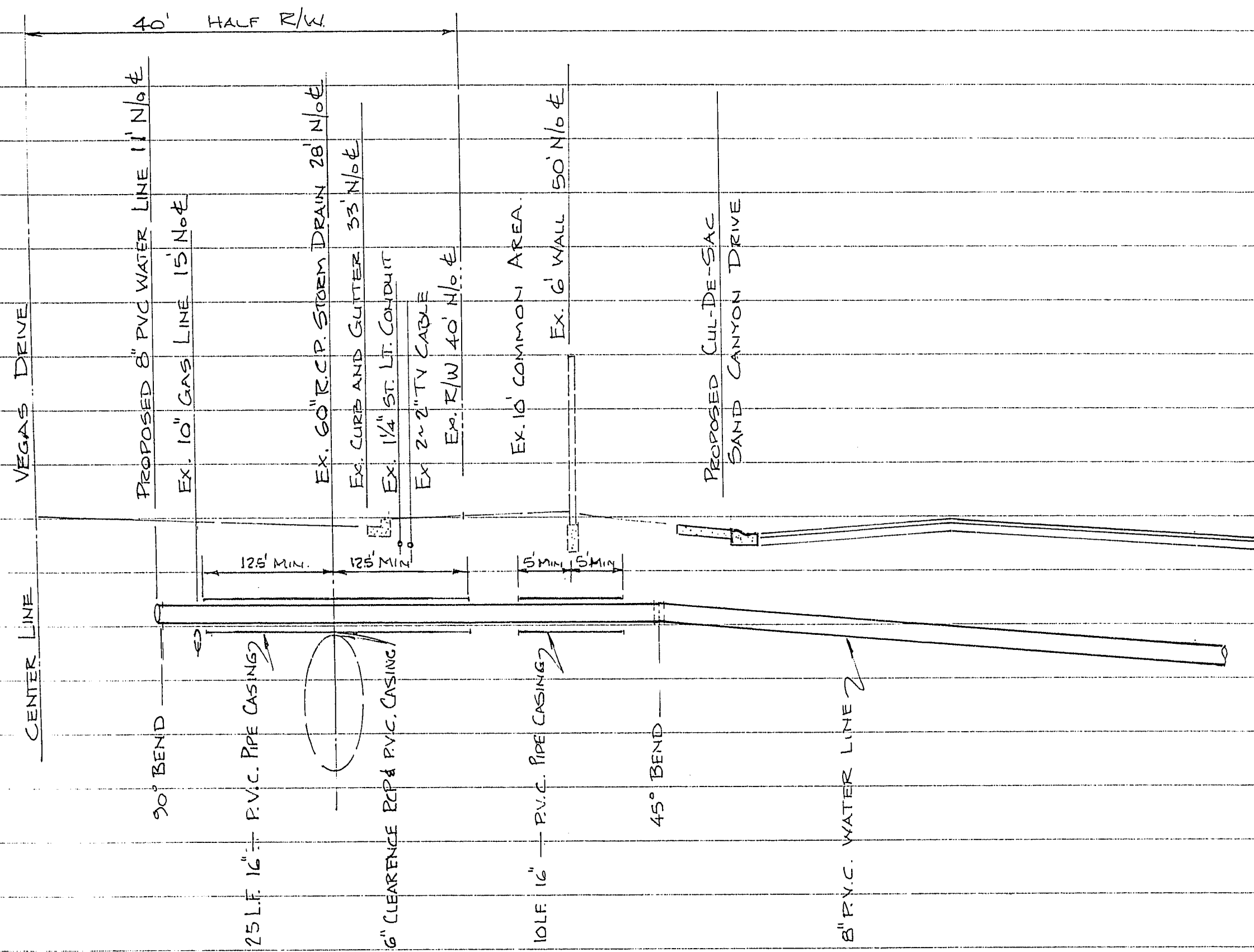
PROFILE OF 8" P. V. C. WATER LINE AND 16" I.D. P. V. C. CASING IN VEGAS DRIVE
