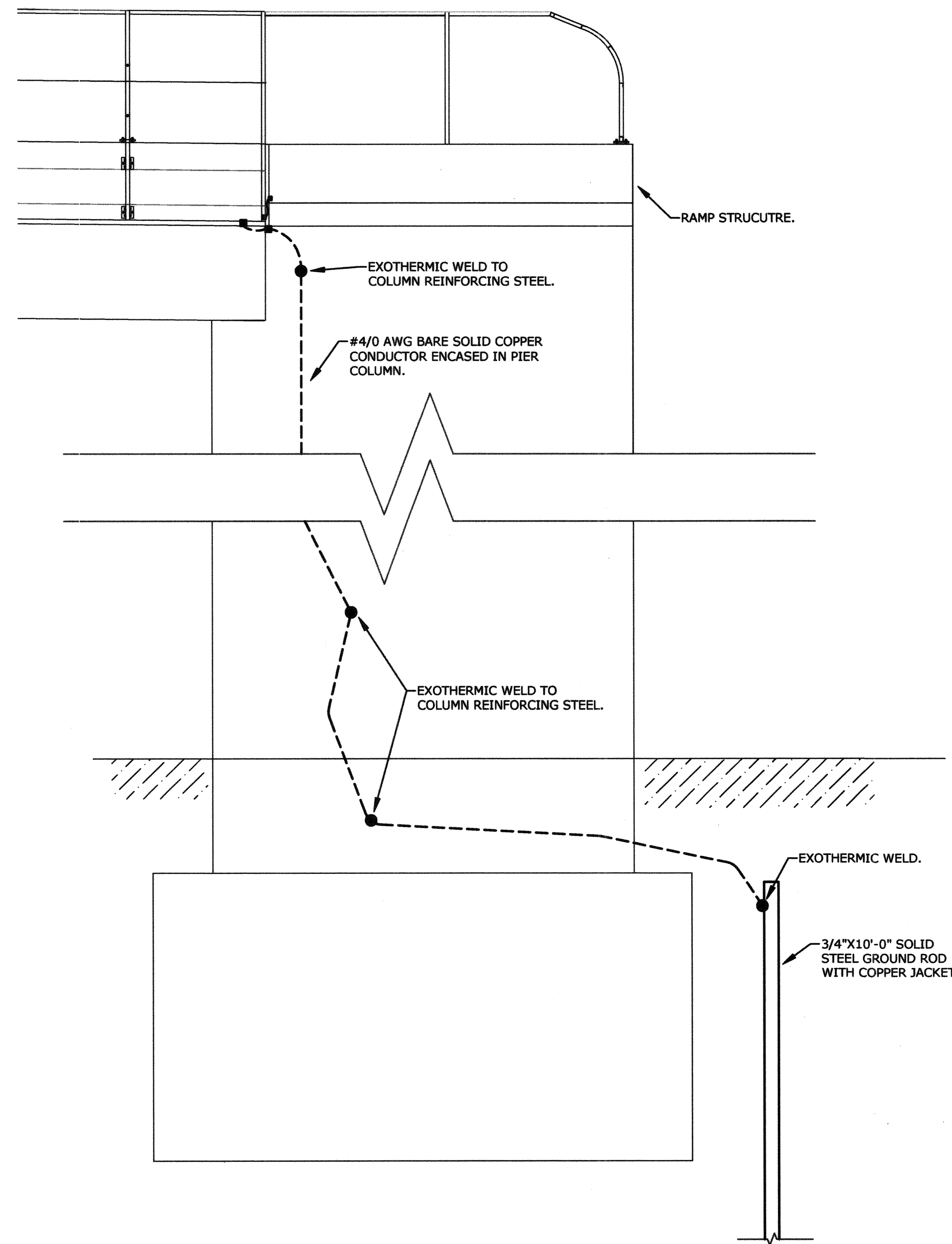
A E0.04 NTS BRIDGE GROUNDING
