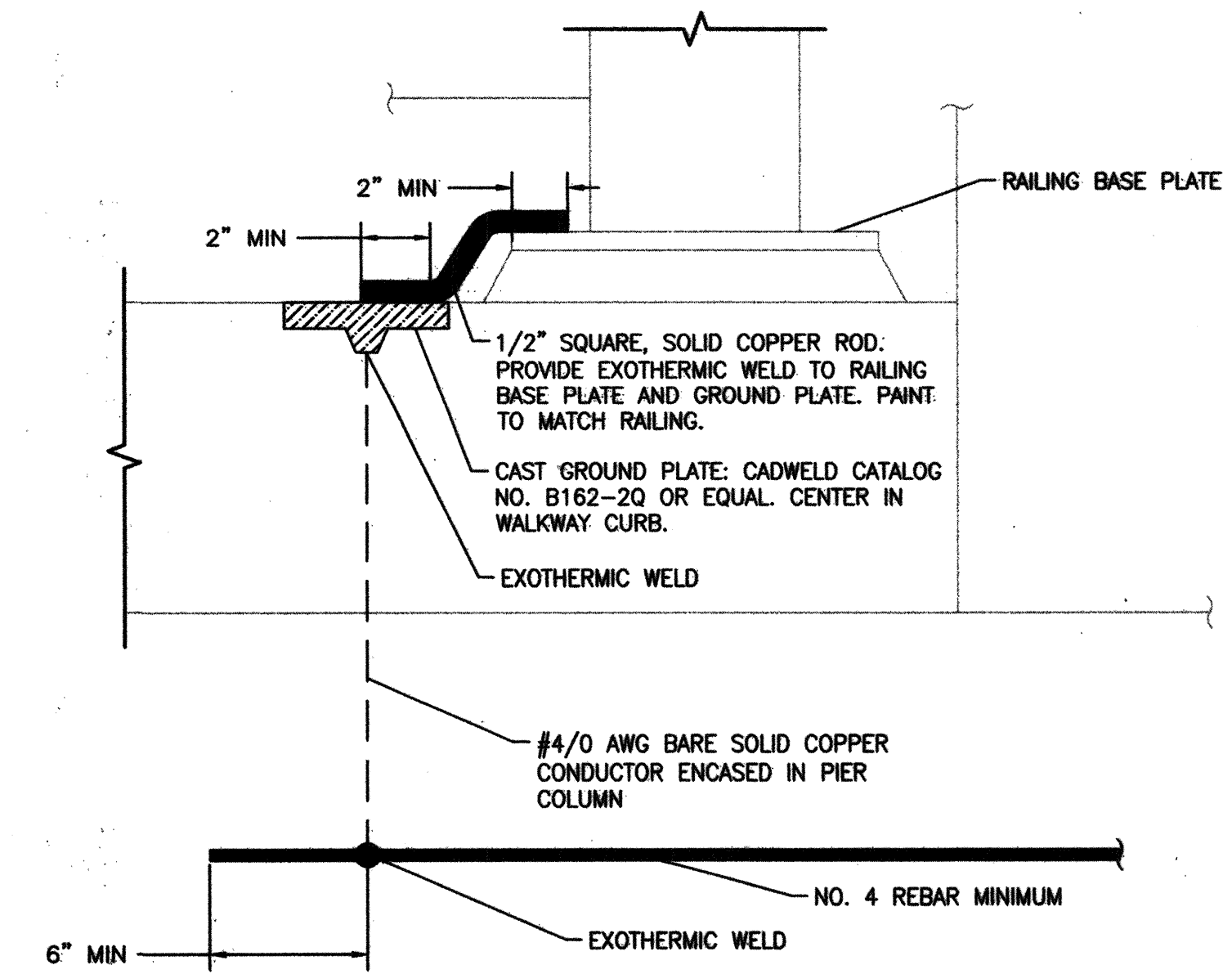
D E0.04 NTS PEDESTRIAN RAIL BONDING DETAIL
