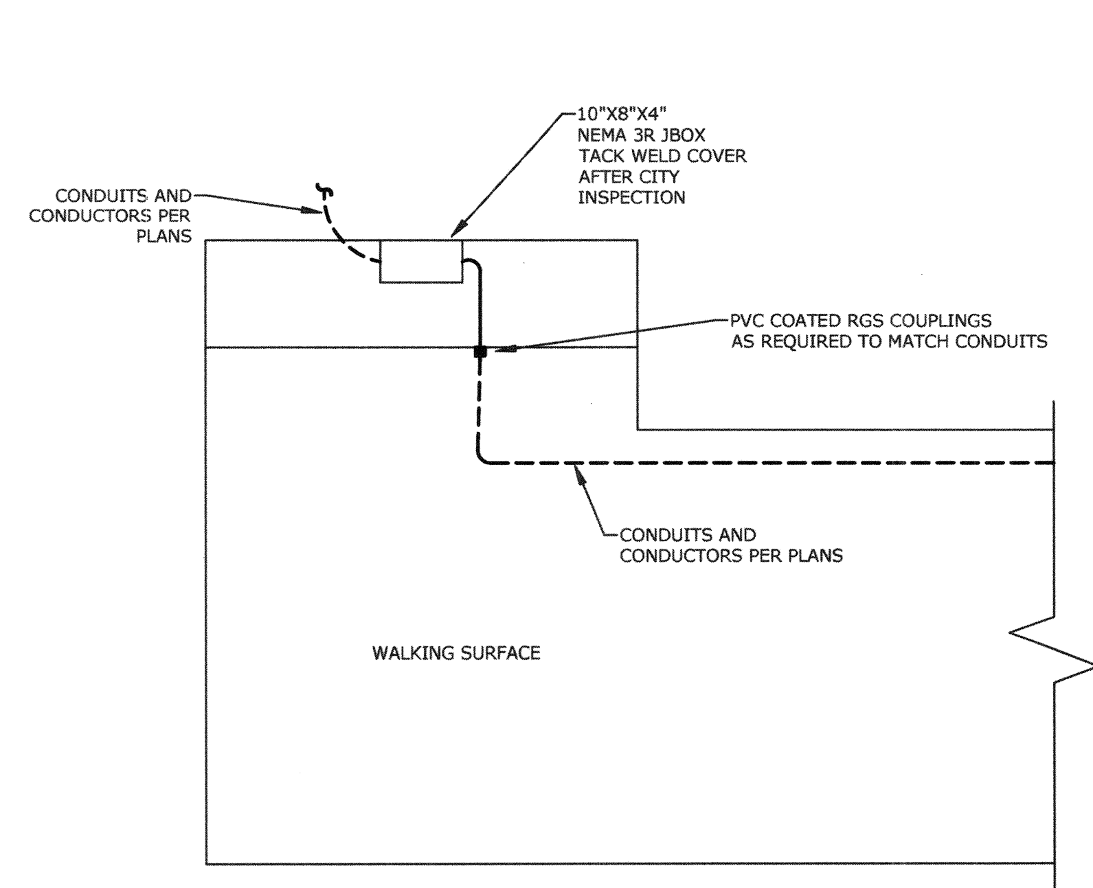
A RAMP TO BRIDGE CONNECTION E0.03 NTS
