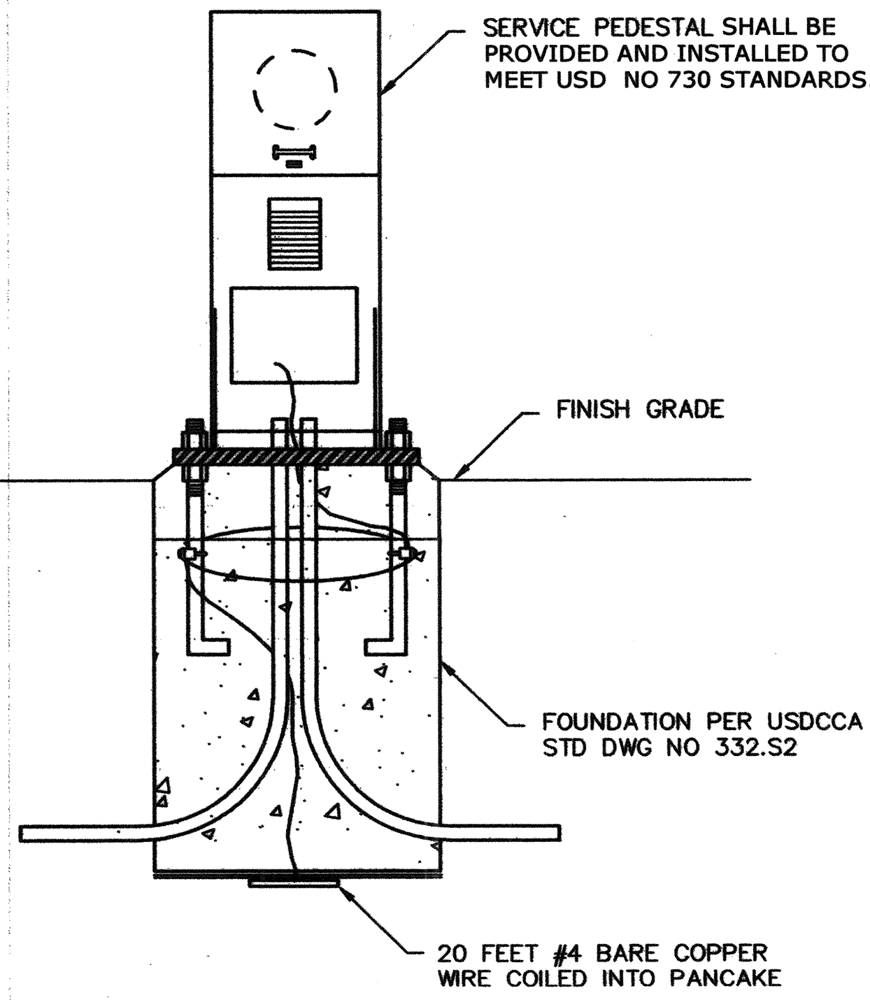
D SERVICE PEDASTAL AND FOUNDATION E0.03 NTS
