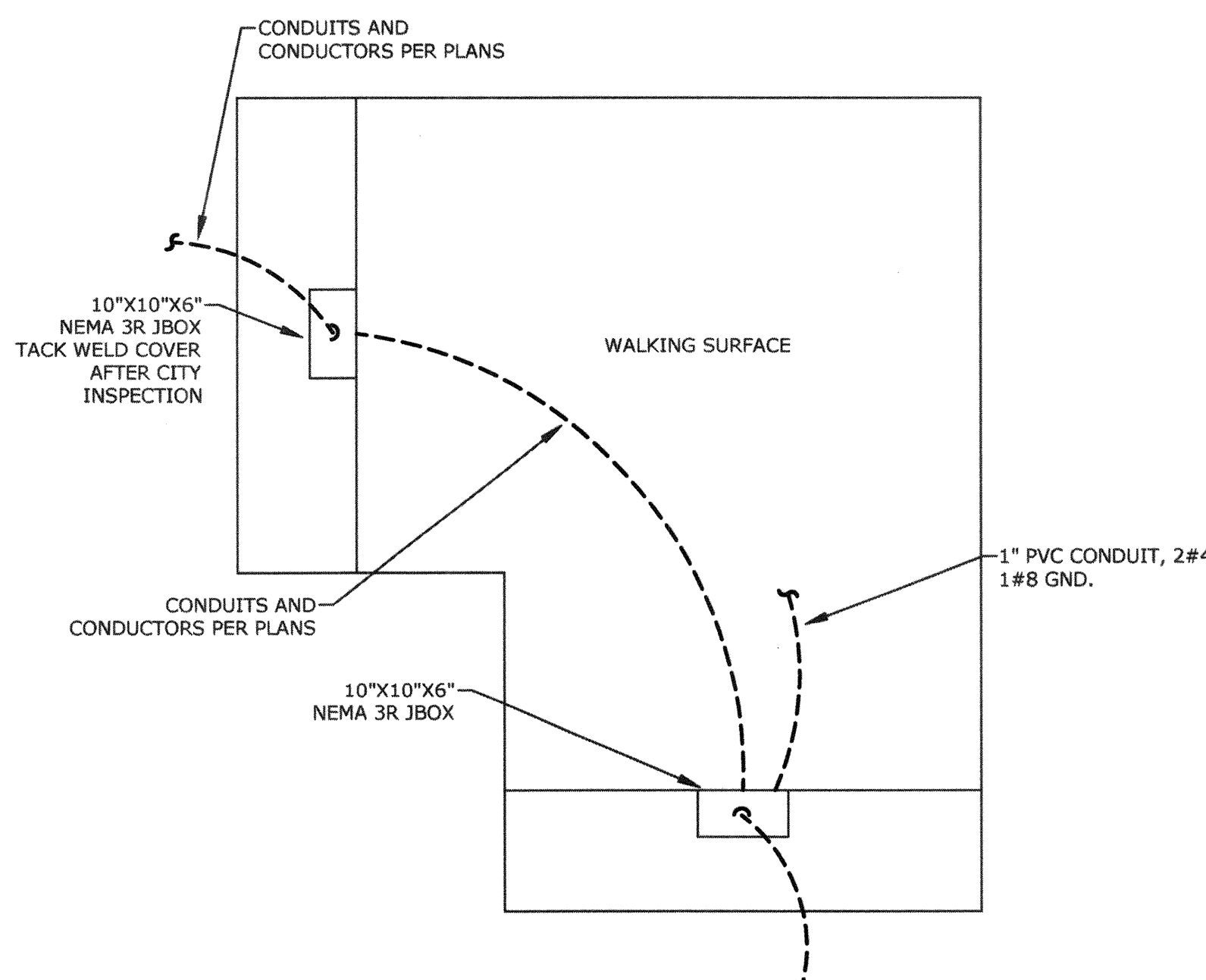
B RAMP TO BRIDGE CONNECTION E0.03 NTS
