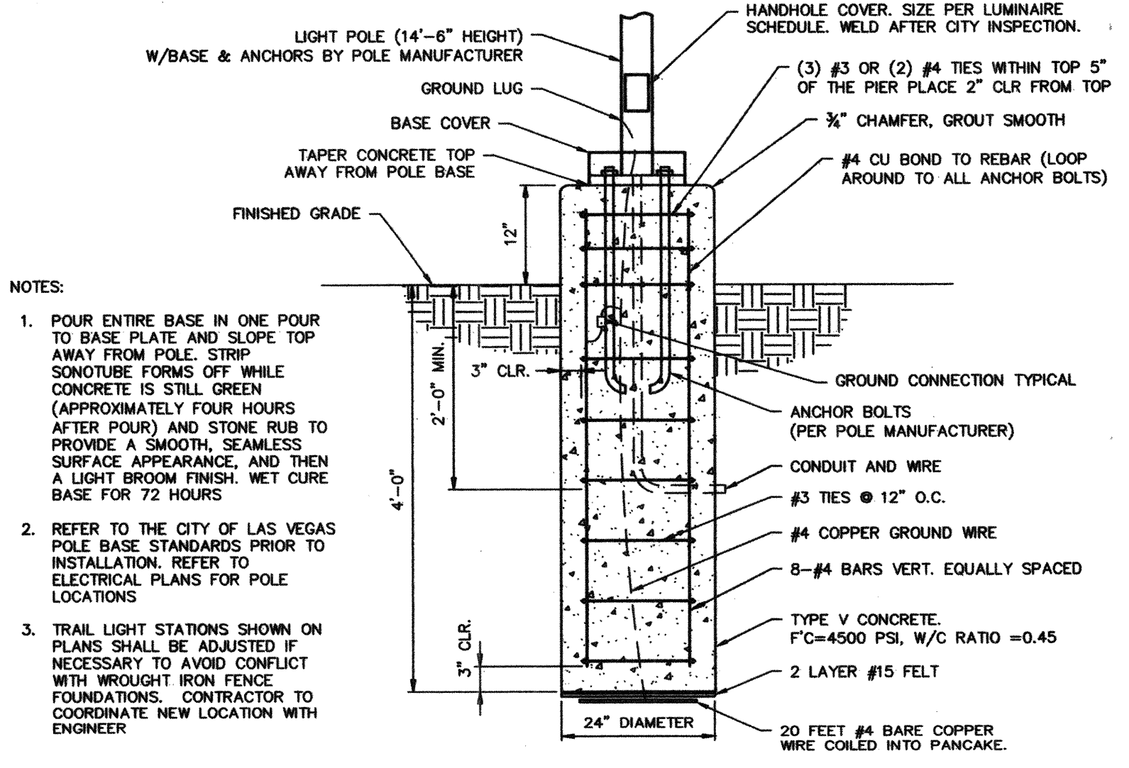
E TRAIL LIGHT POLE ASSEMBLY FOOTING E0.03 NTS
