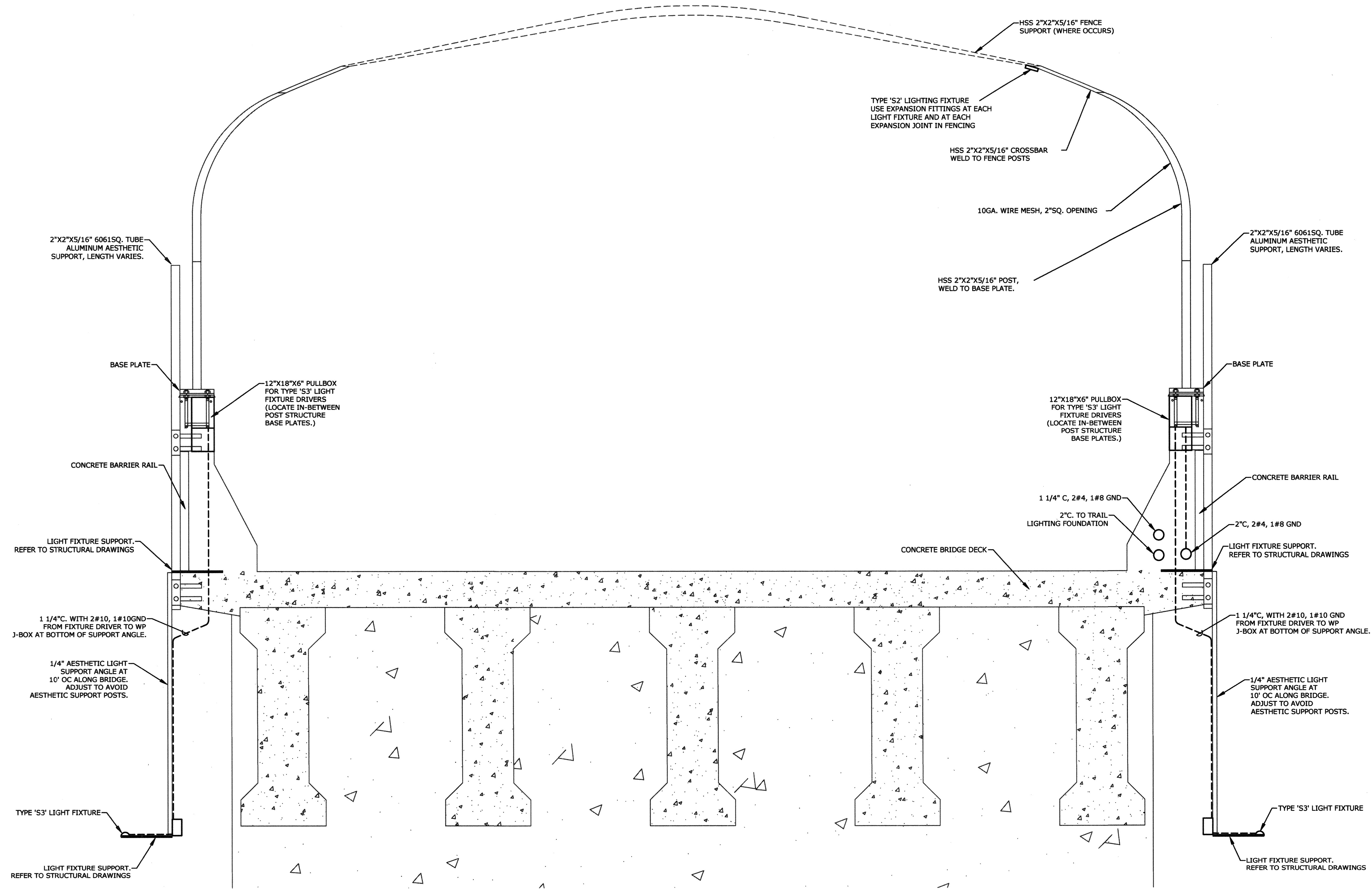
A TYPICAL BRIDGE SECTION E0.02 NTS
