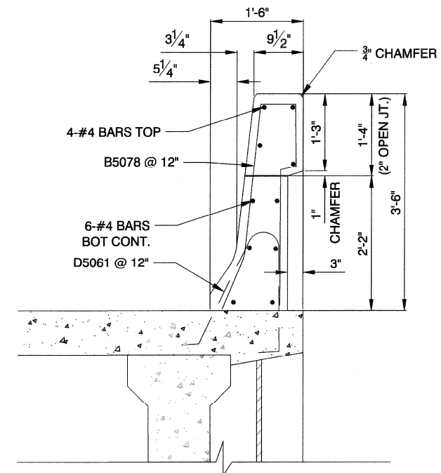
BARRIER RAIL DETAIL
