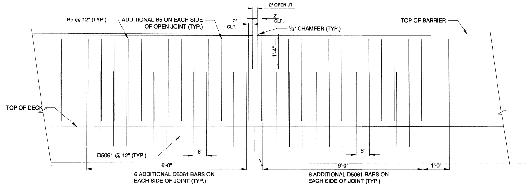
2" OPEN JOINT DETAIL
