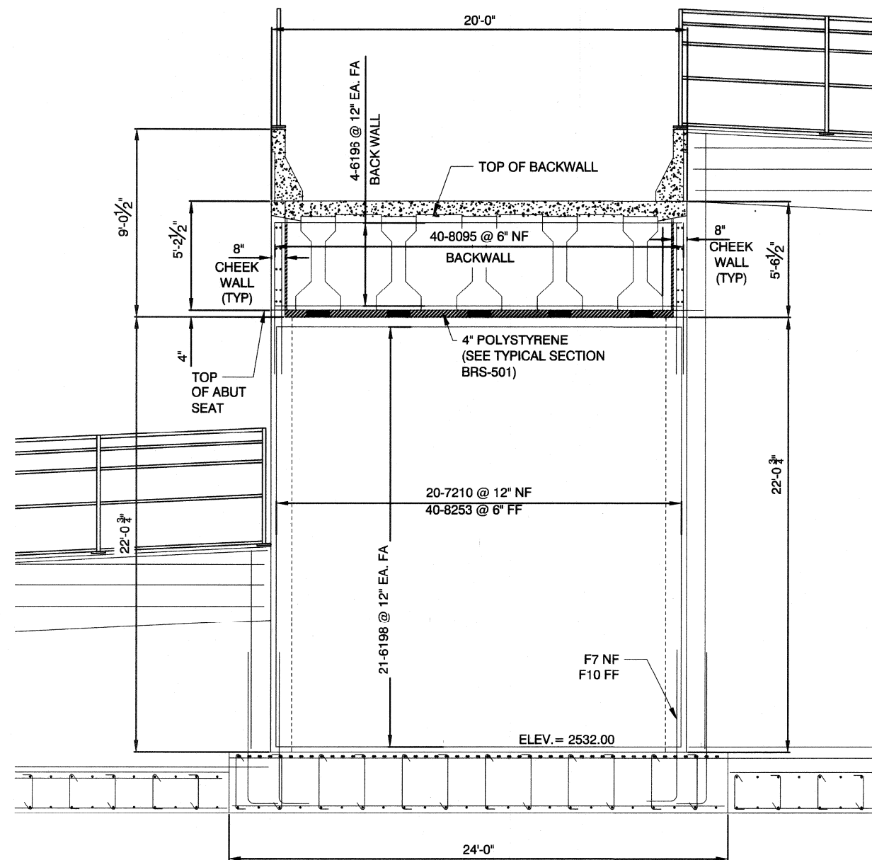
ABUTMENT 1 ELEVATION
