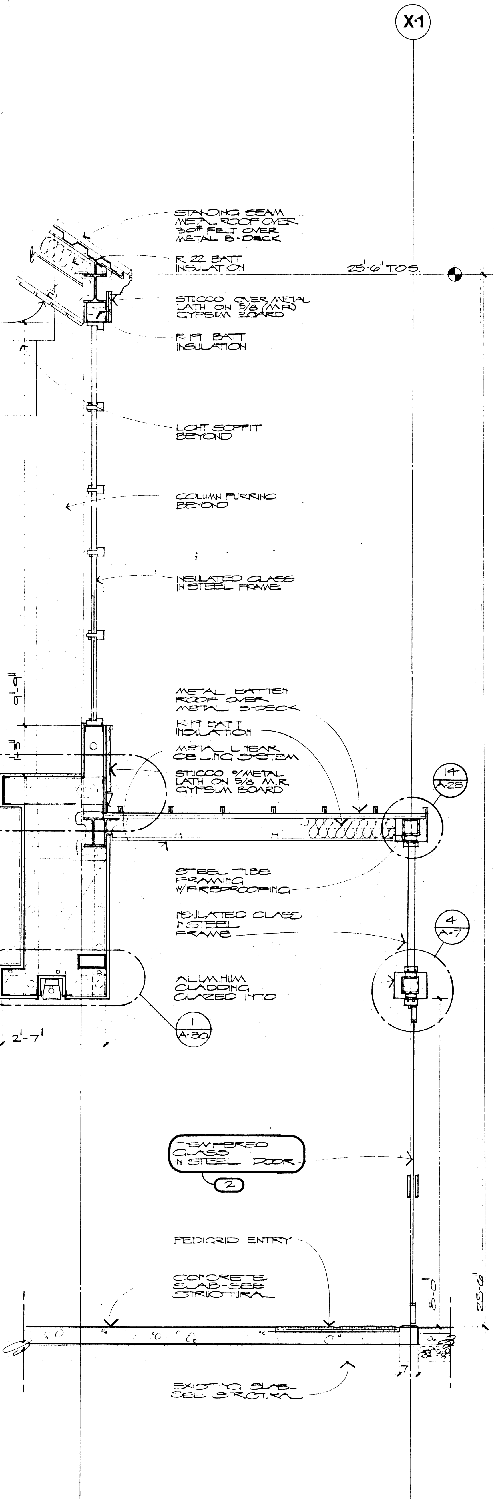
WALL SECTION SCALE 3/4" : 1'-0" 18 A-24
