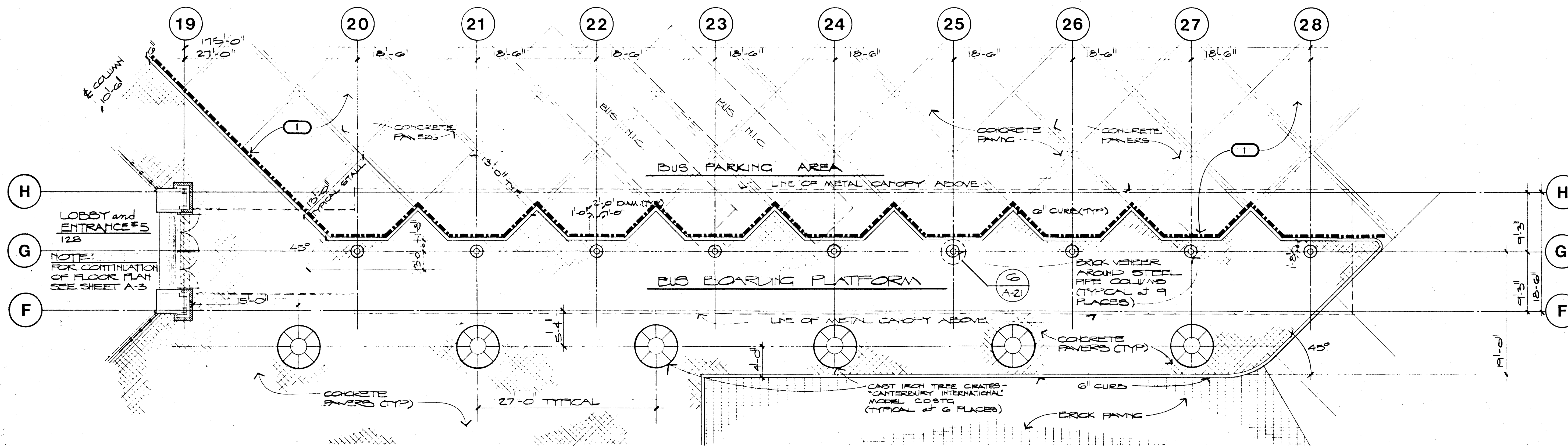
FLOOR PLAN
