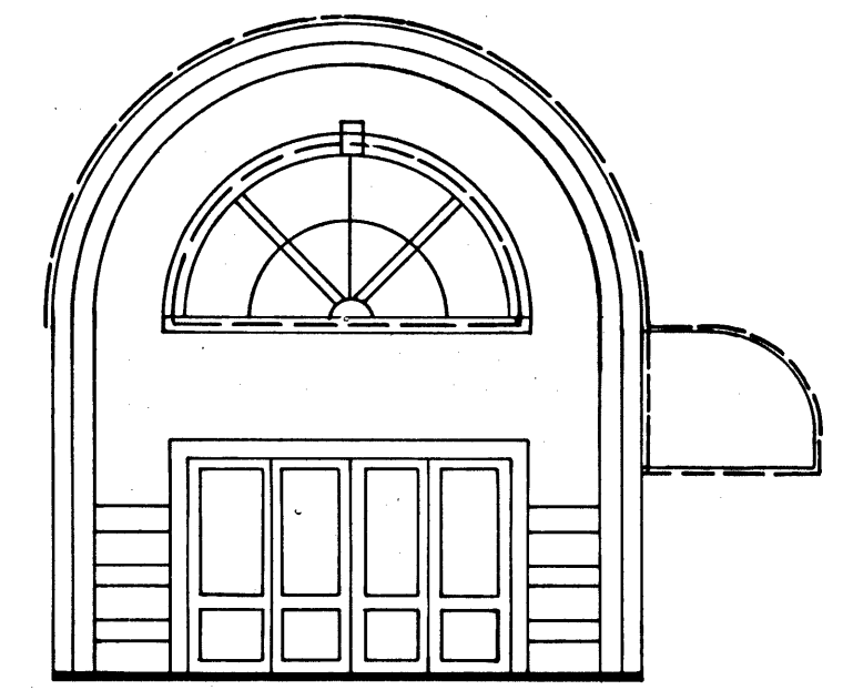
3 TYPICAL ARCH- 6 REQUIRED SCALE: 1/8" = 1'-0" 3
