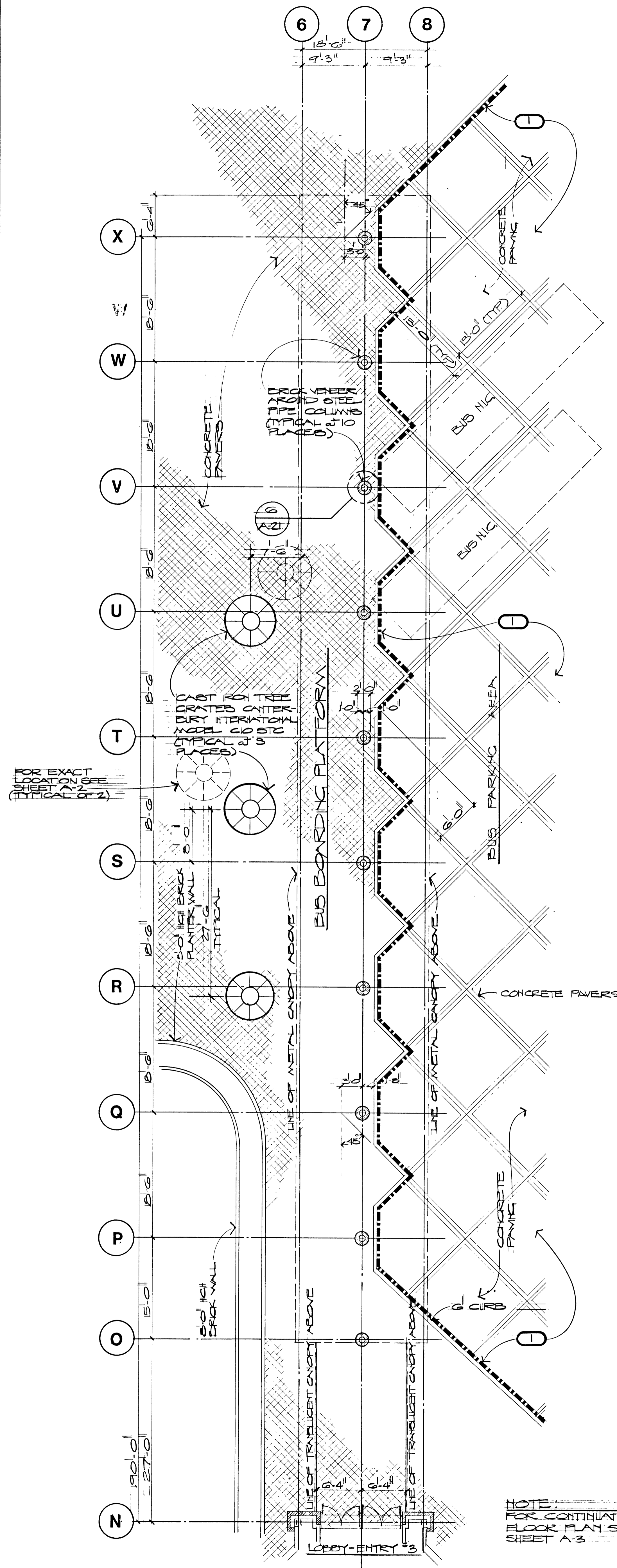
FLOOR PLAN
