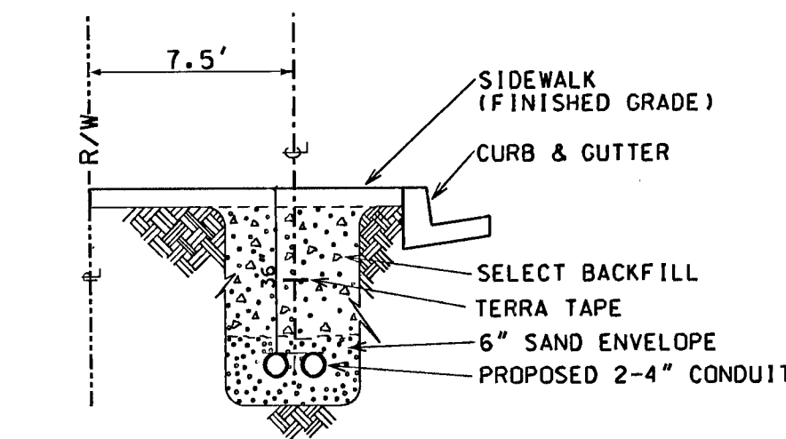
A TRENCH DETAIL A WITH SIDEWALK
