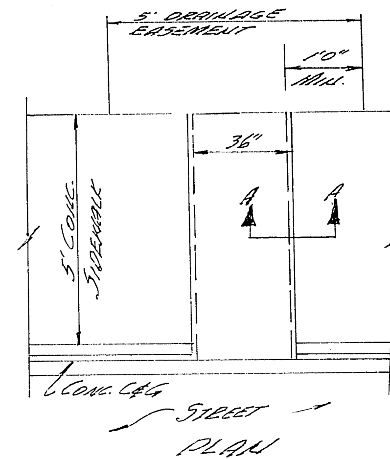
SIDWALK DRAIN NO SCALE
