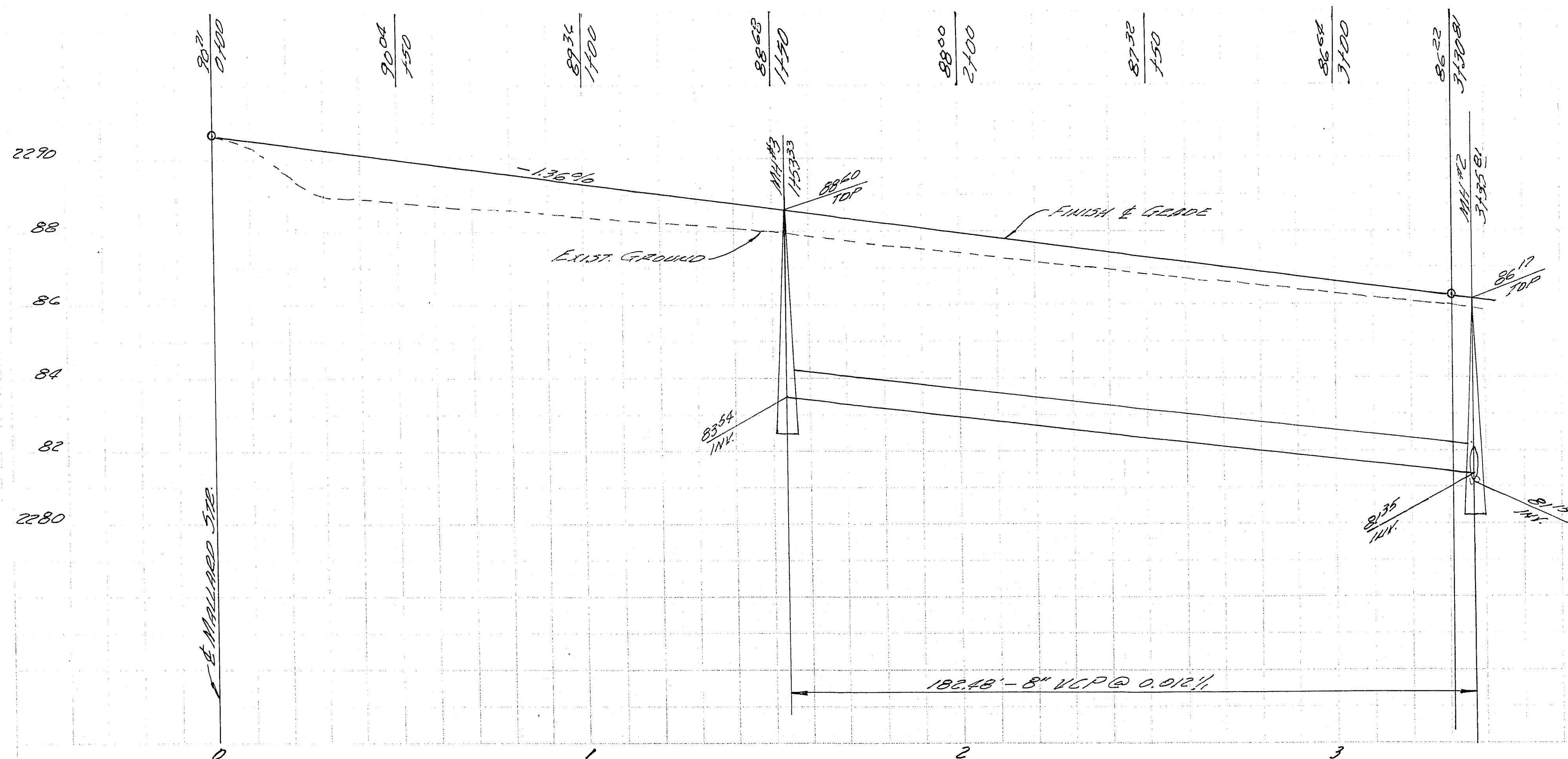
CONCERT DRIVE SCALES: H. 1" = 20' V. 1" = 2'
