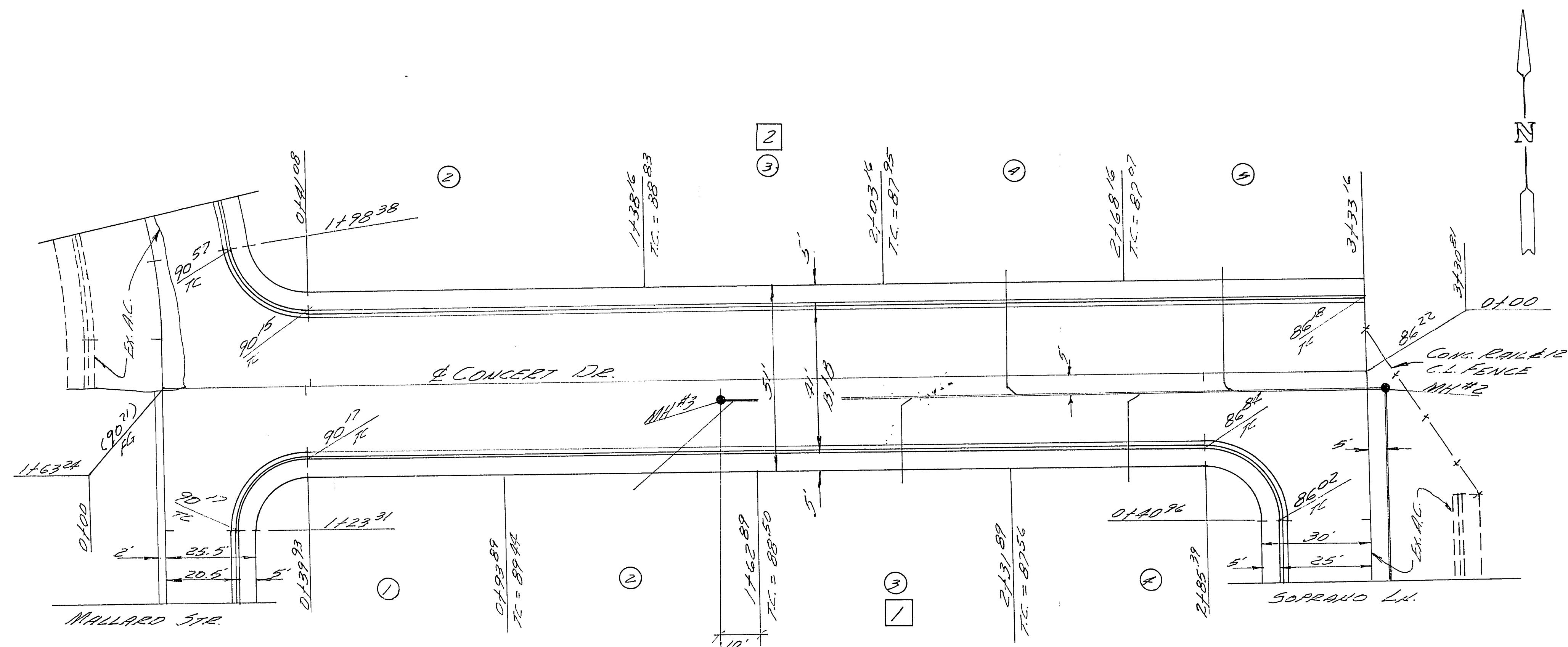
CONCERT DRIVE SCALES: H. 1" = 20' V. 1" = 2'
