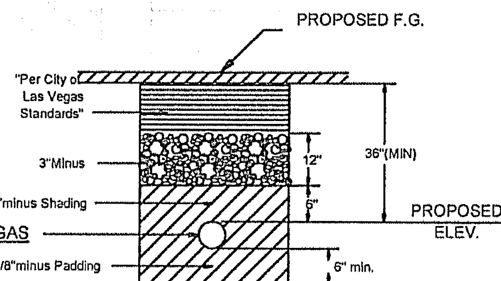
CLV TRENCH DETAIL PER RTC STD
