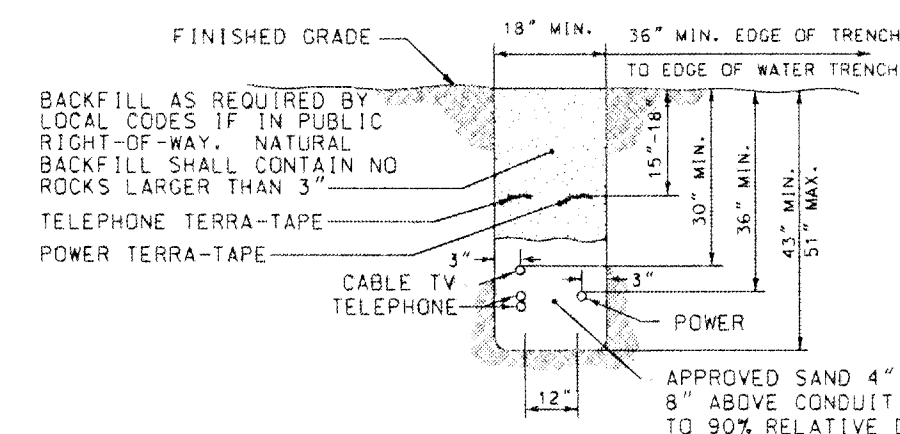
ONSITE TRENCH DETAIL
