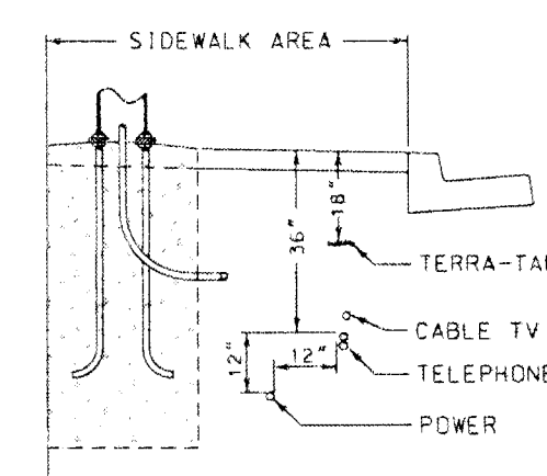
OFFSITE TRENCH DETAIL
