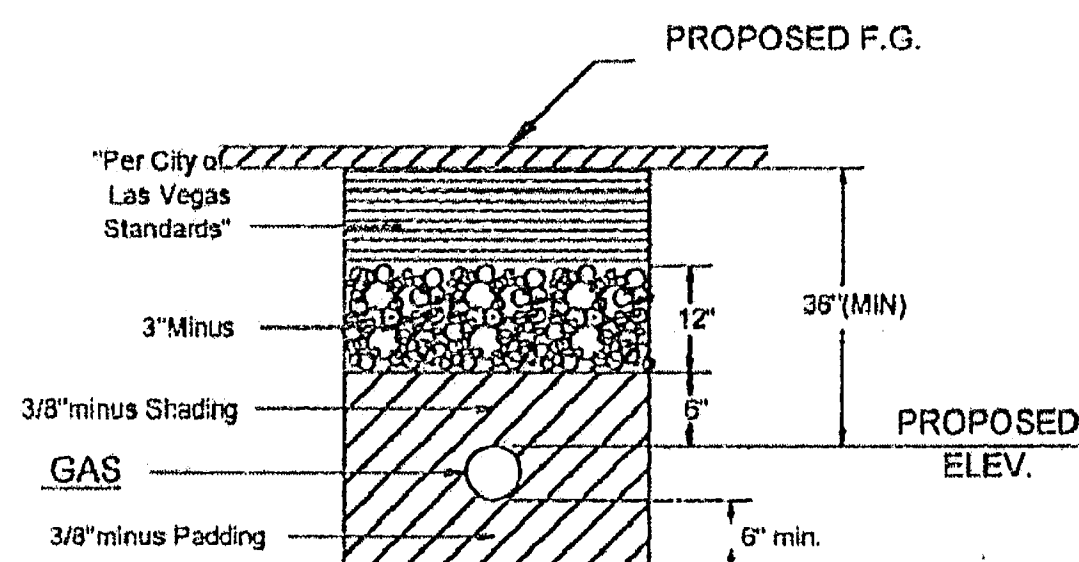
CLV TRENCH DETAIL
