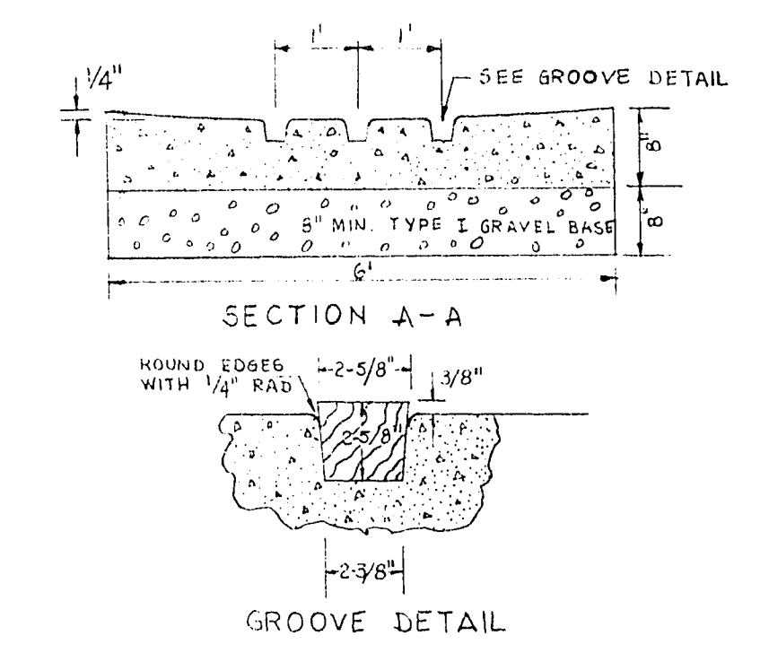
VALLEY GUTTER DETAIL
