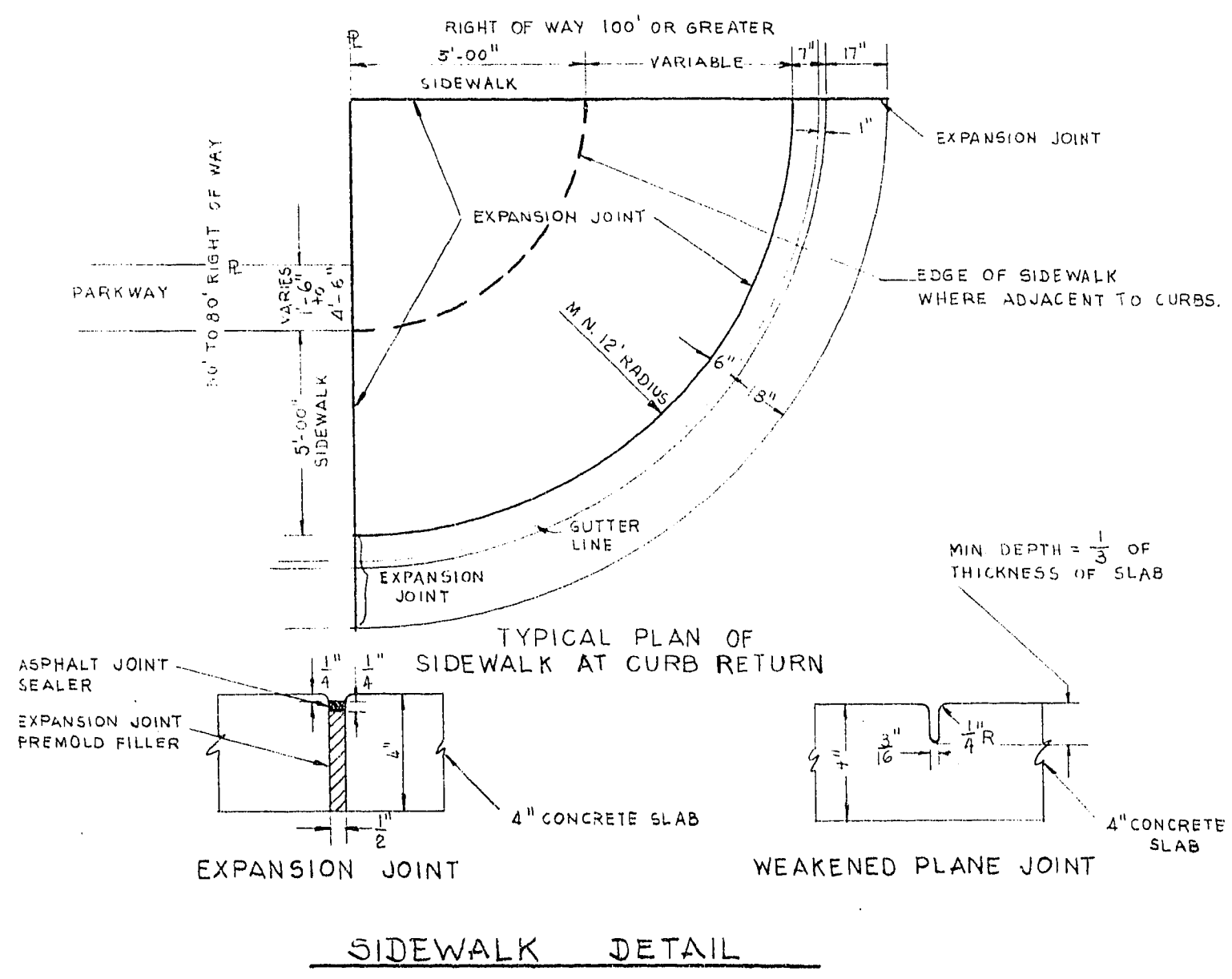
SIDEWALK DETAIL
