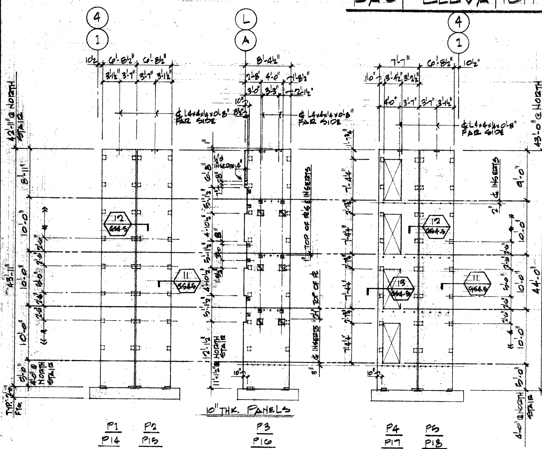
NORTH & SOUTH STAIRS ELEVATION
