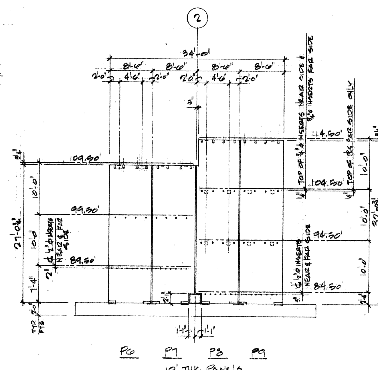
SOUTH ELEVATION @ GRID F
