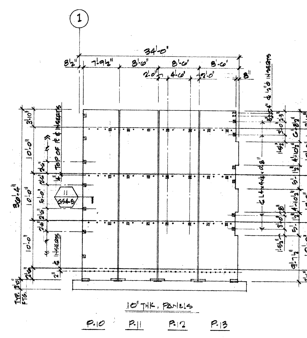
SOUTH ELEVATION @ GRID L
