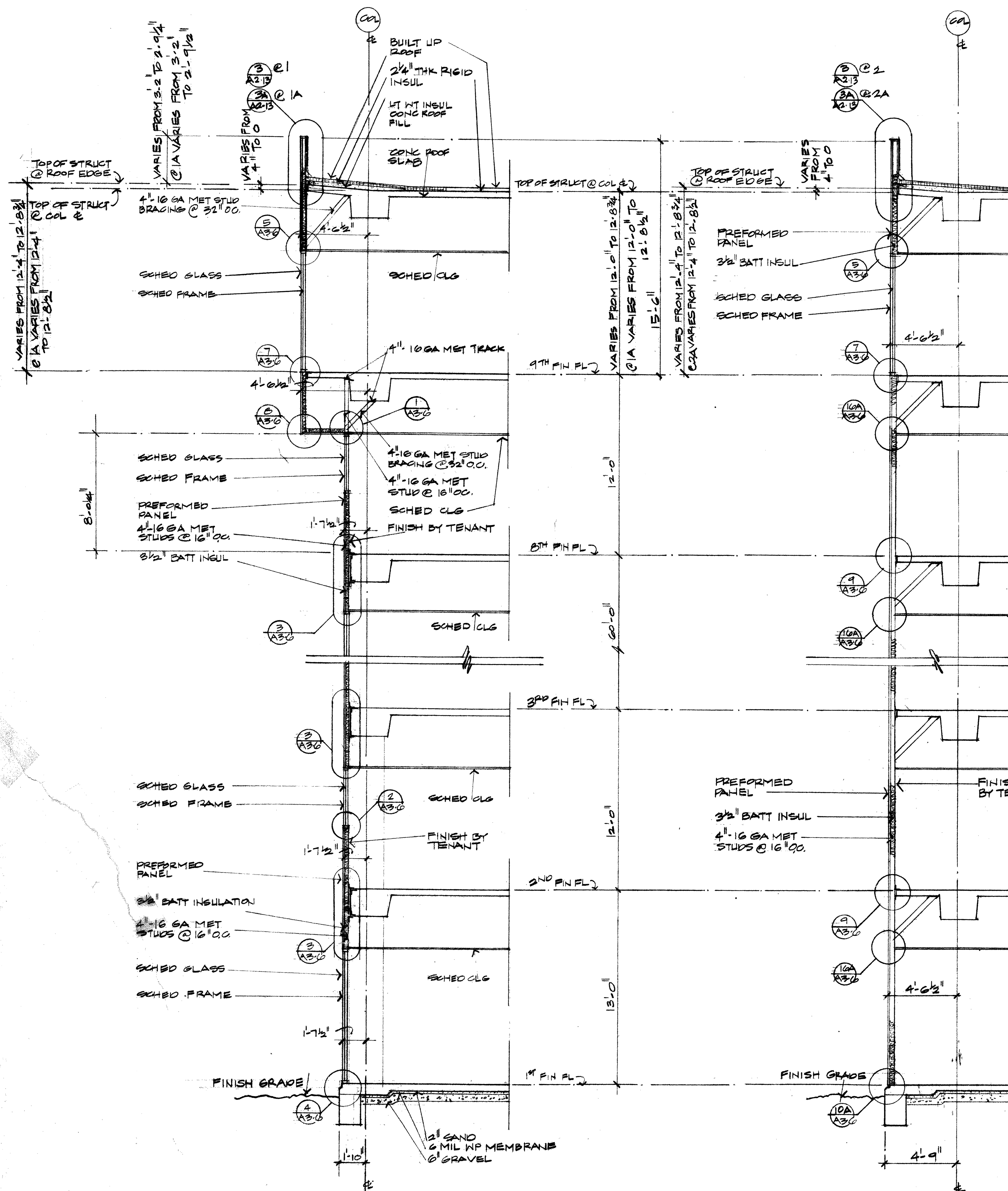
① 1A SECTION 1/4" = 1'-0"
