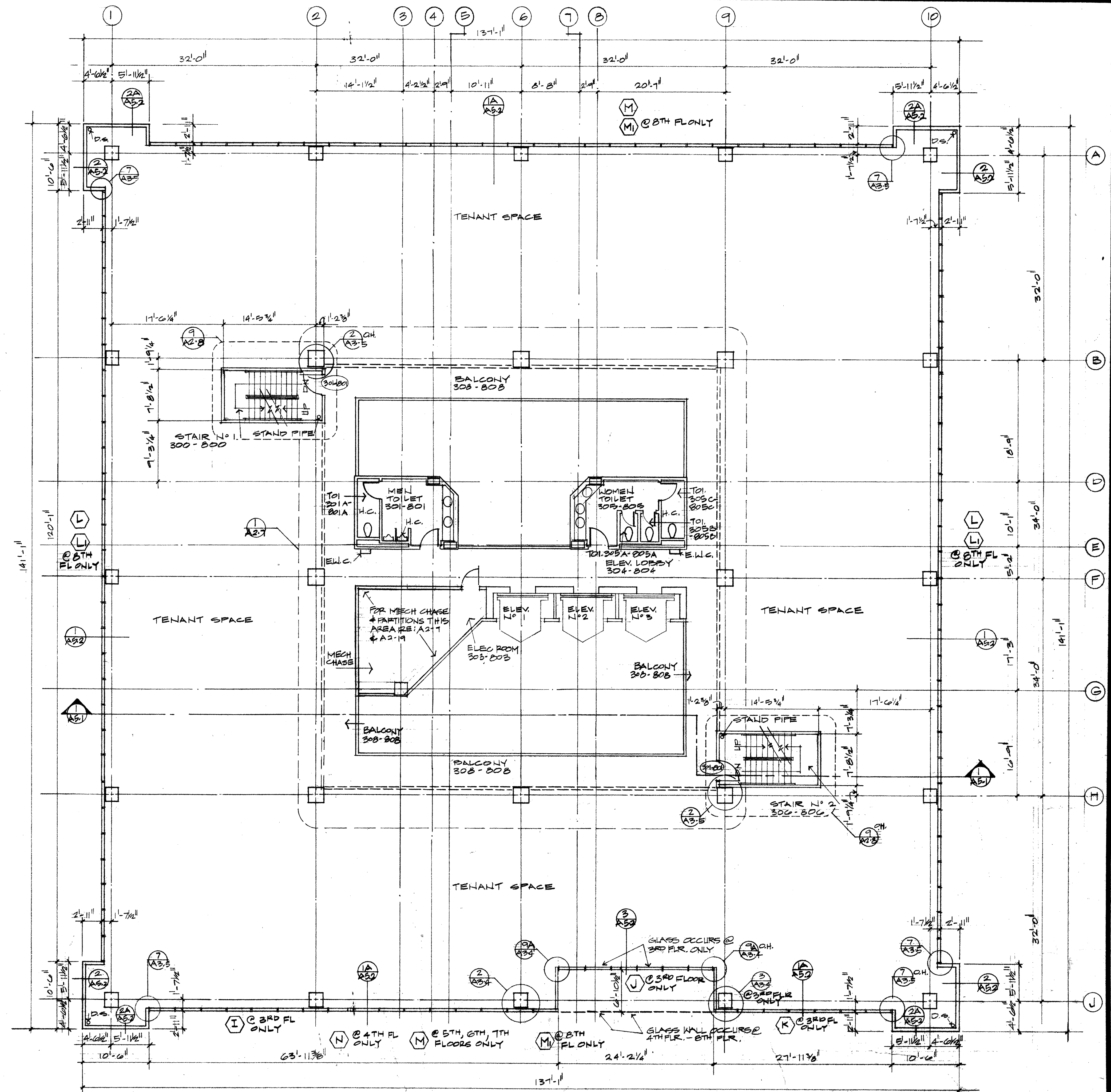
① THIRD THRU EIGHTH FLOOR PLAN 1/8" = 1'-0"
