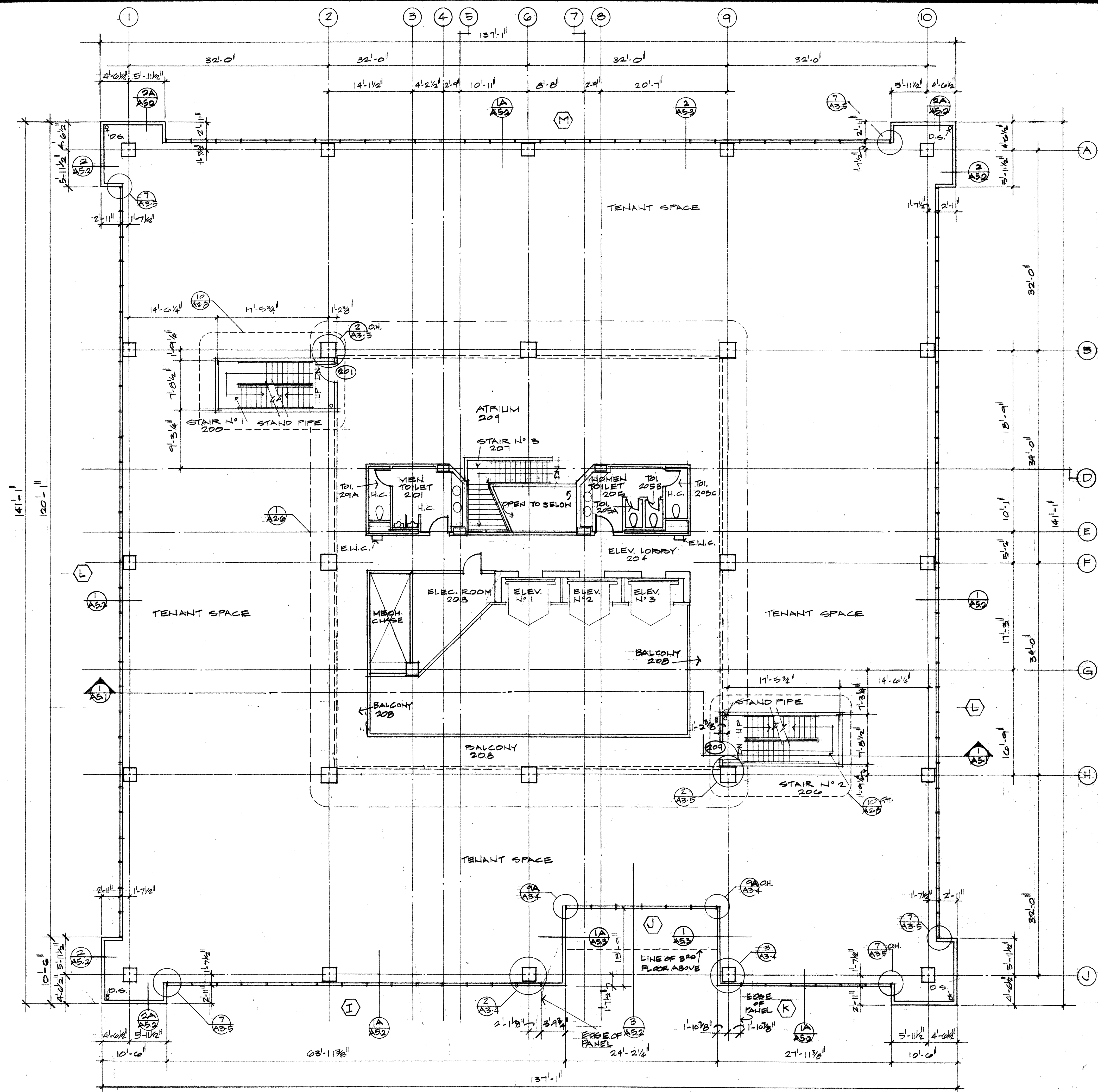
① SECOND FLOOR PLAN \frac{1}{8}'' = 1'-0''
