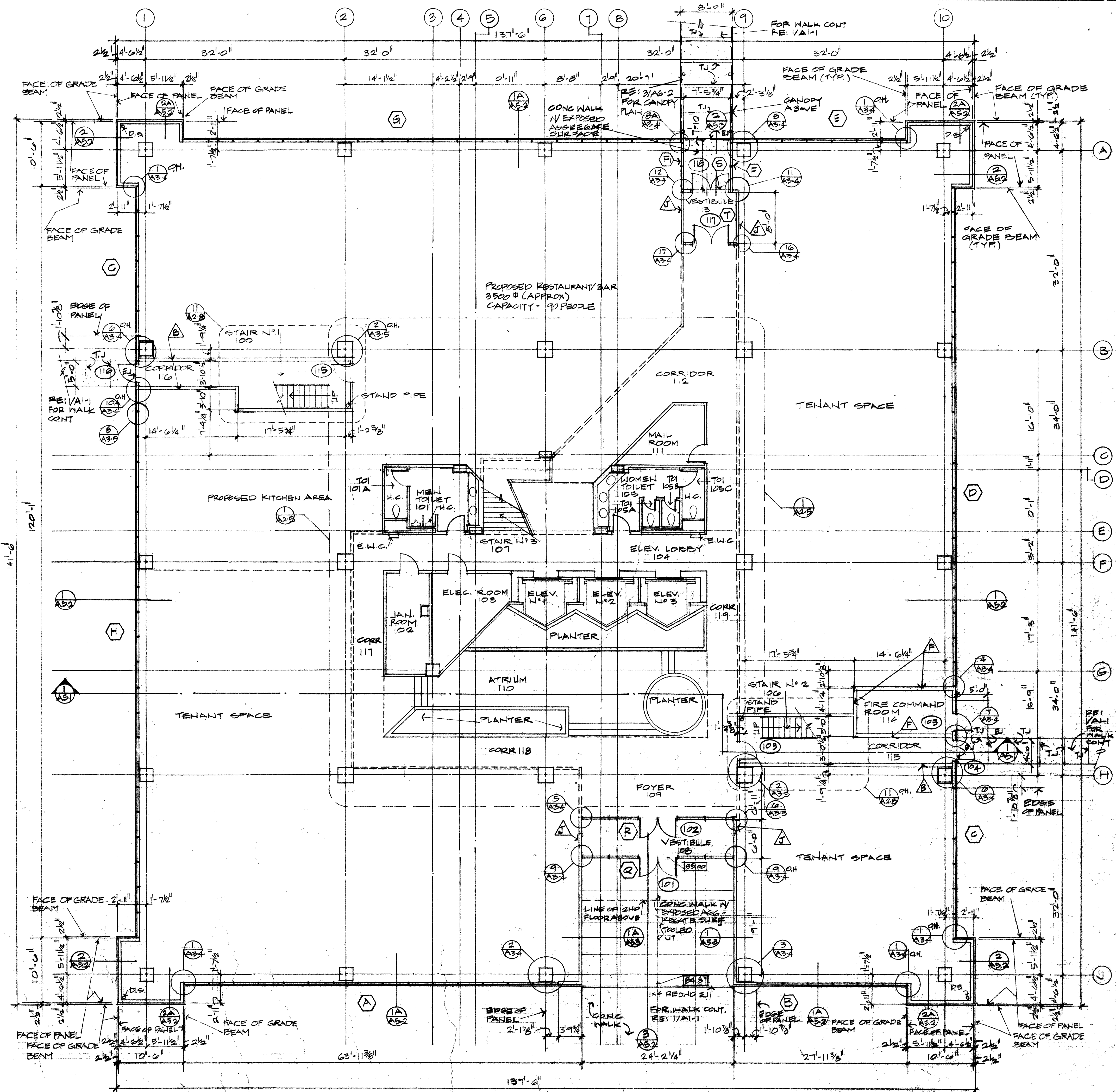
① FIRST FLOOR PLAN 1/8" = 1'-0"
