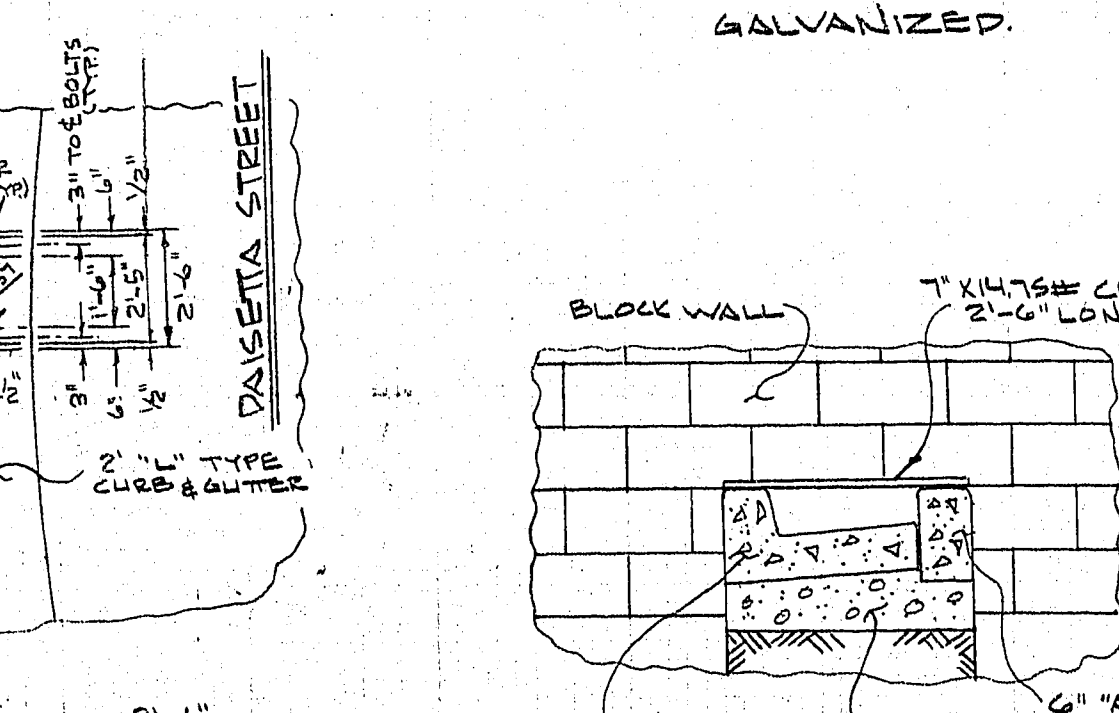
DETAIL "B"
