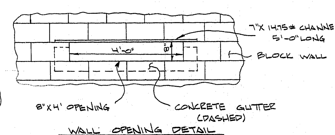
DETAIL "B"
