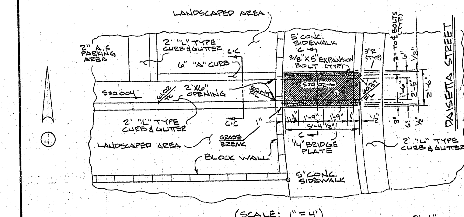
DETAIL "B"
