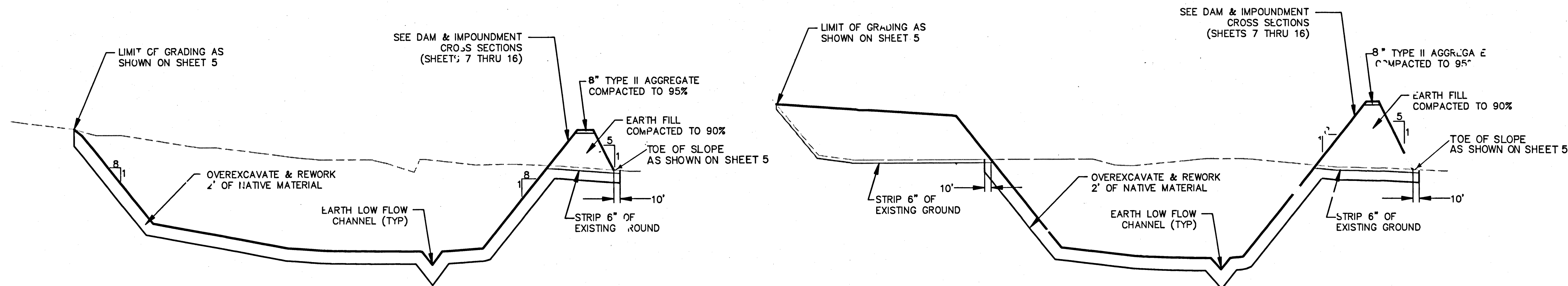
TYPICAL CROSS SECTION (limit of grading in fill)
