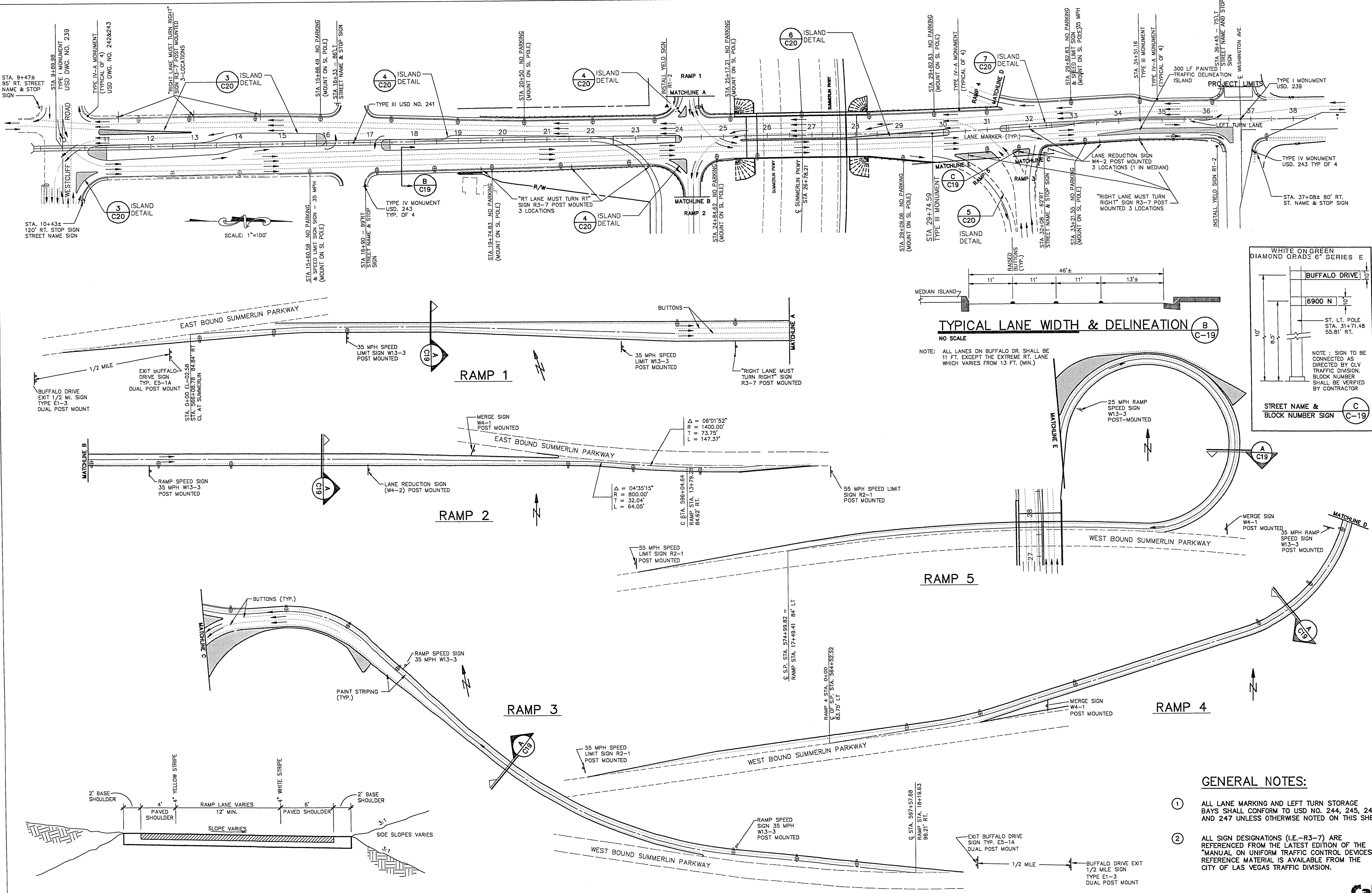
TRAFFIC STRIPING SIGNING & MONUMENTATION PLAN 1" = 100'
