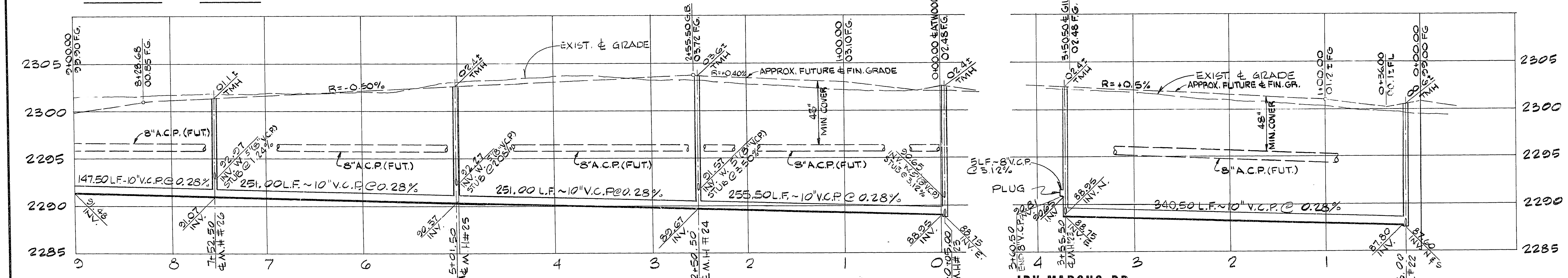
PROFILE SCALE: HORIZ. 1"=50' VERT. 1"=5'
