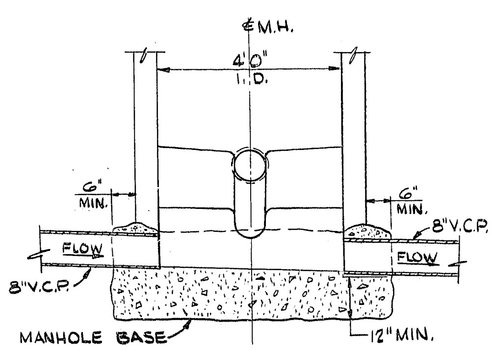
SECTION 1 MANHOLE DETAIL FOR M.H. NOS. 23 THRU 29, 35 THRU 32 & NO. 42
