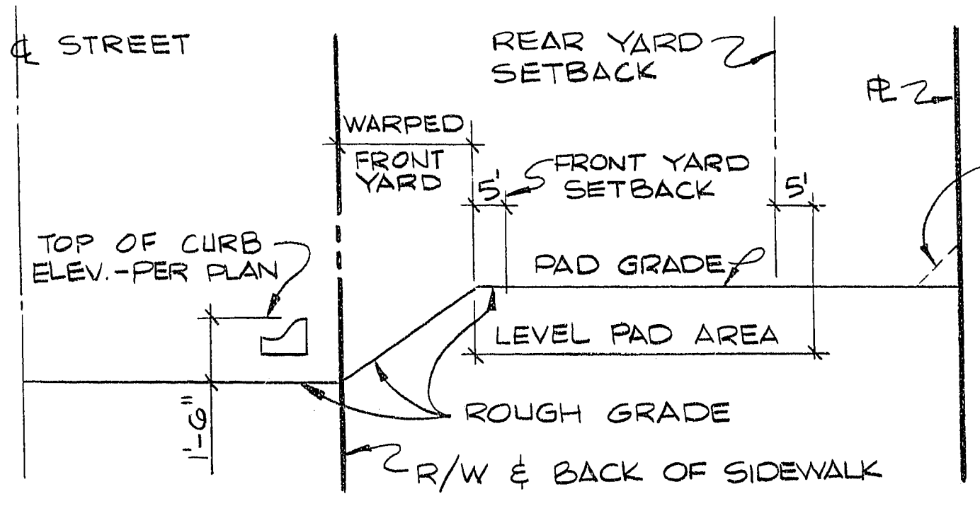
TYPICAL ROUGH GRADING
