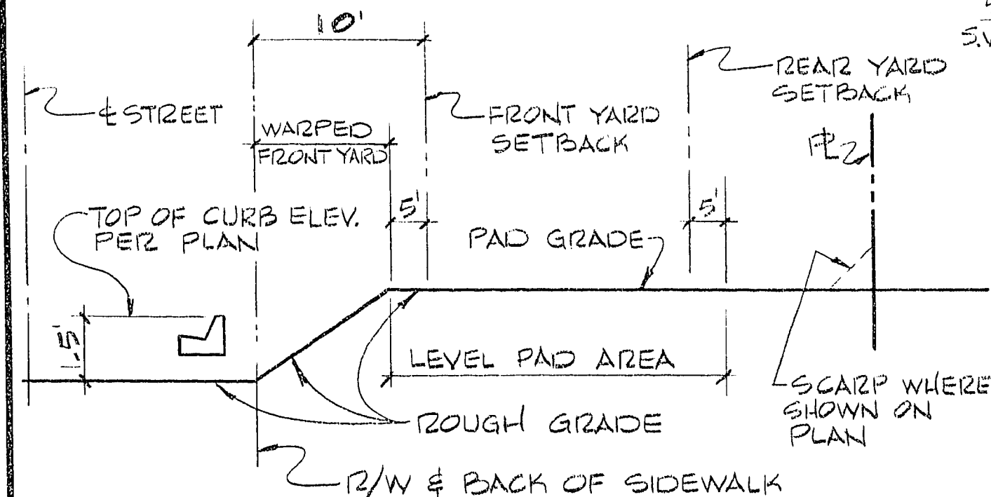
TYP. ROUGH GRADING
