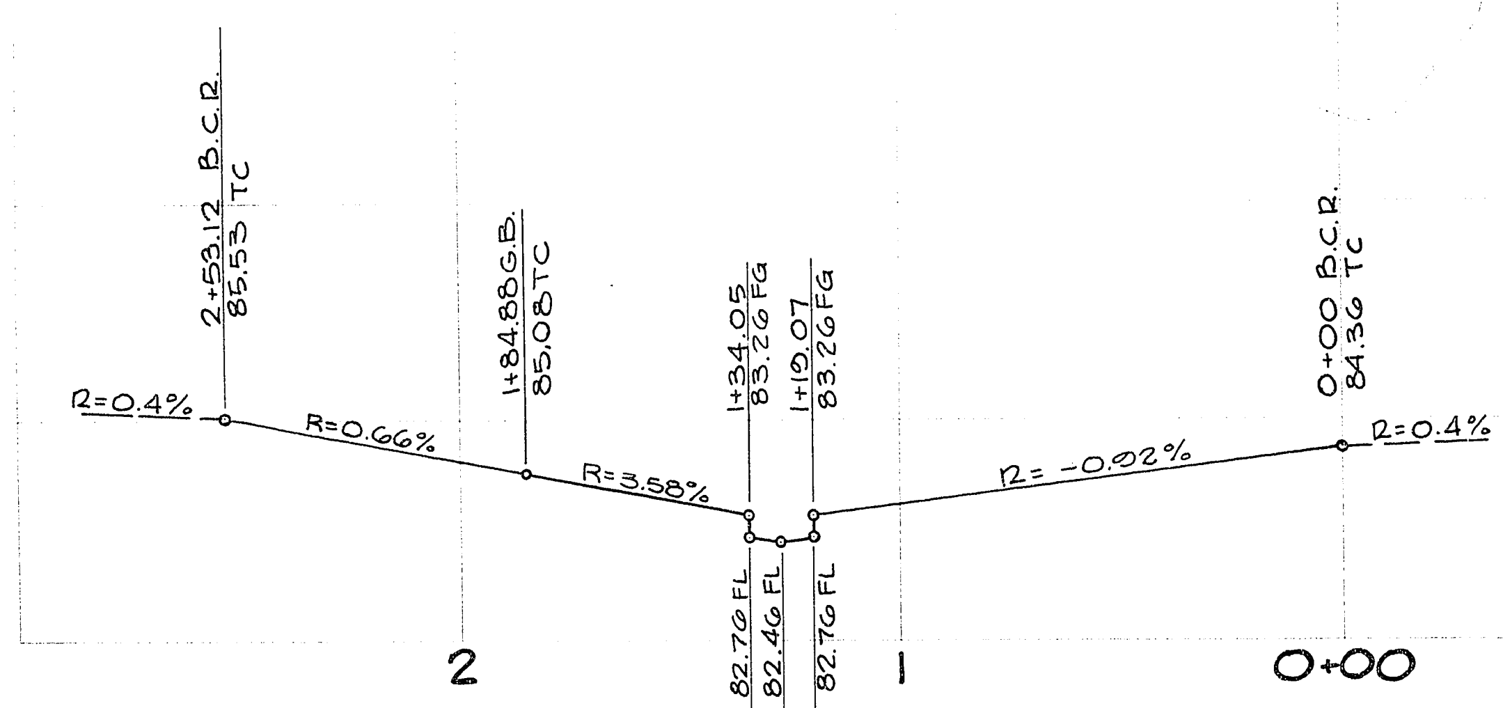
CUL-DE-SAC PROFILE
