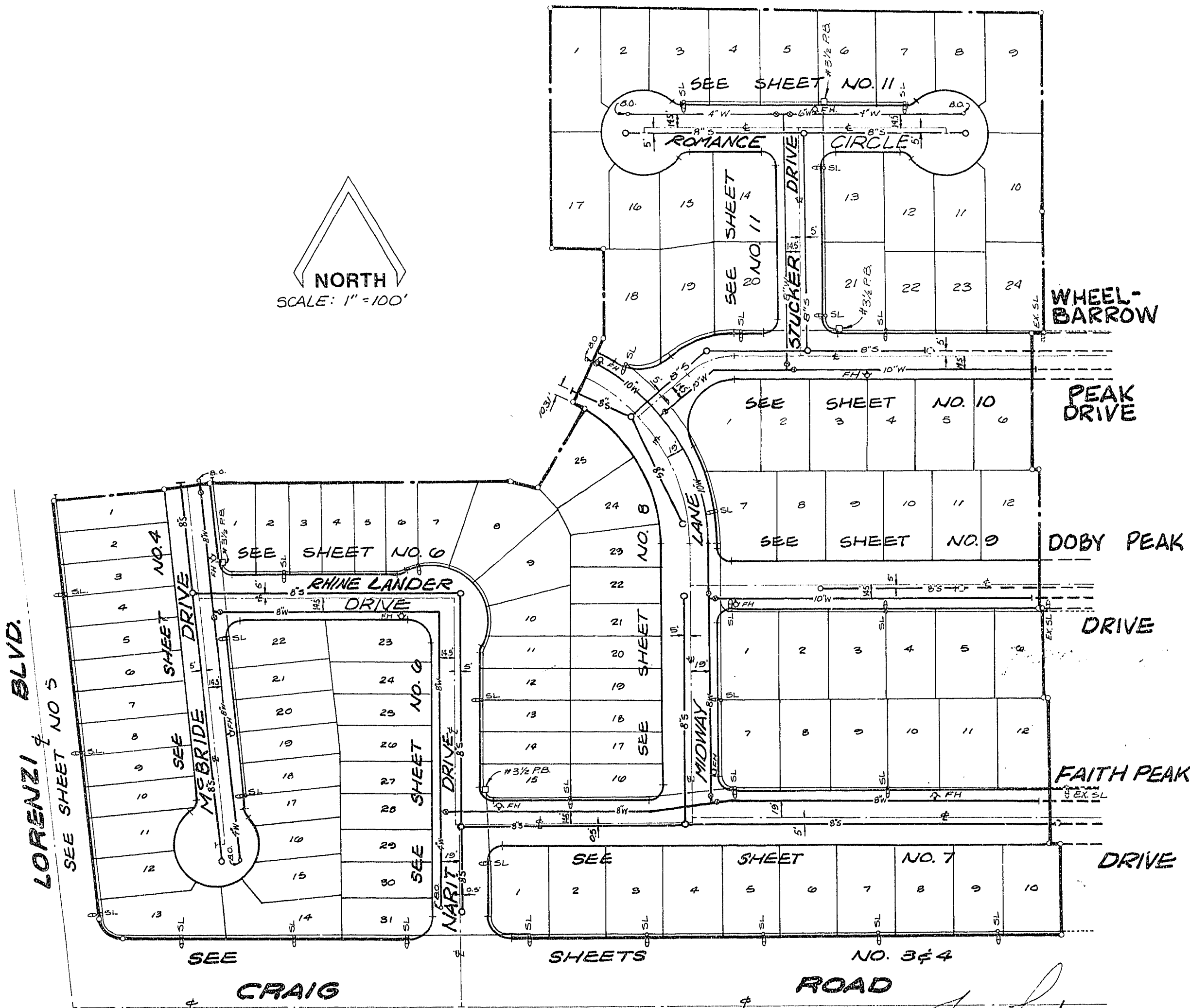
SHEET INDEX & OVERALL UTILITY PLAN
