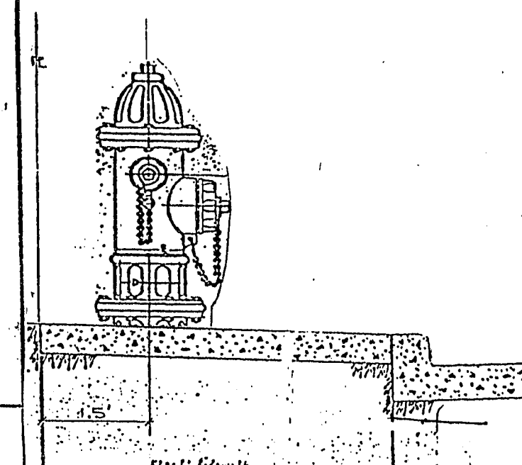
STANDARD FIRE HYDRANT DETAIL City Of Las Vegas
