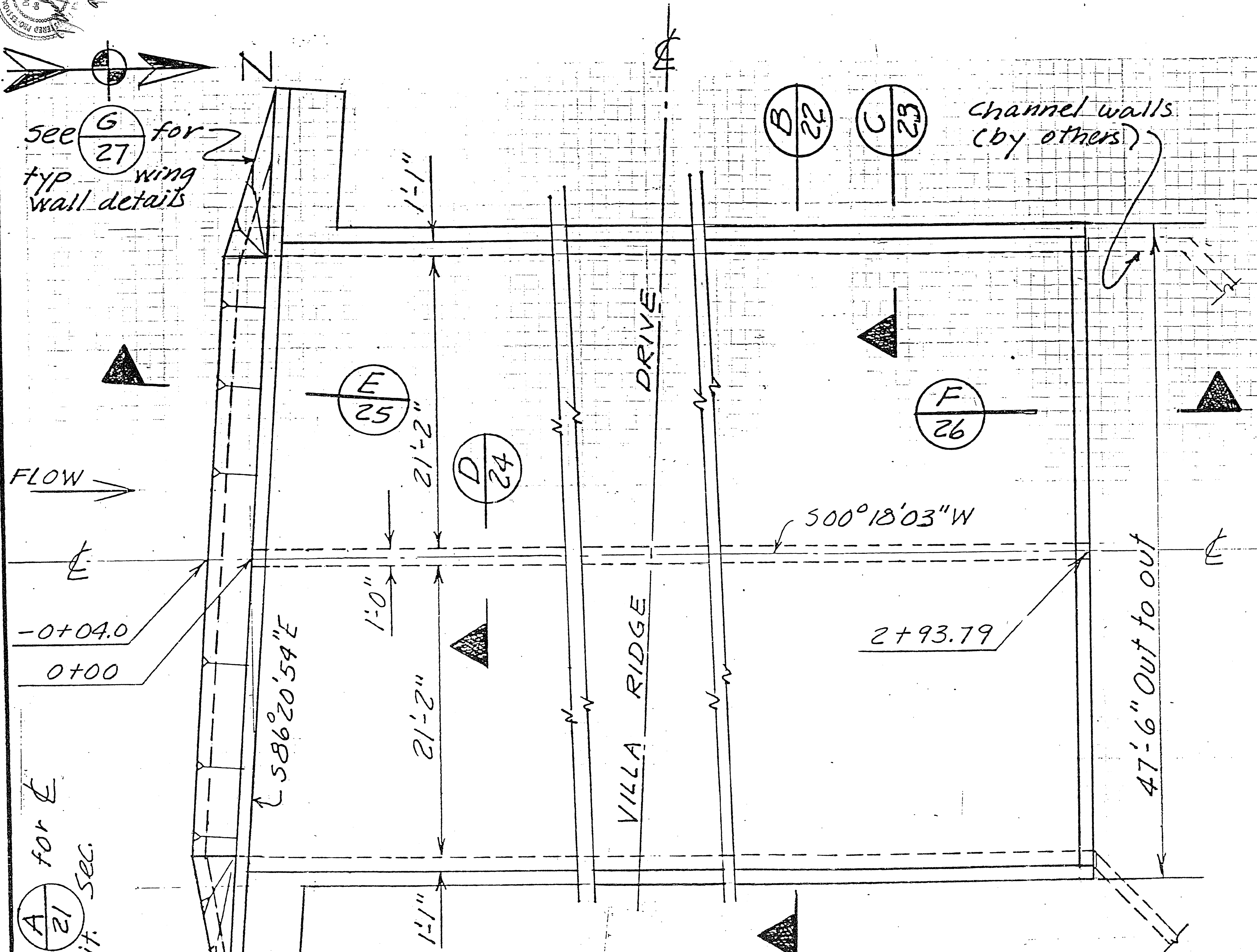
PLAN - ARCH CULVERT @ 27+51.72 VILLA RIDGE DRIVE Scale 1"=10'
