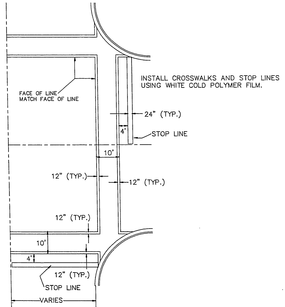
CROSSWALK DETAIL
