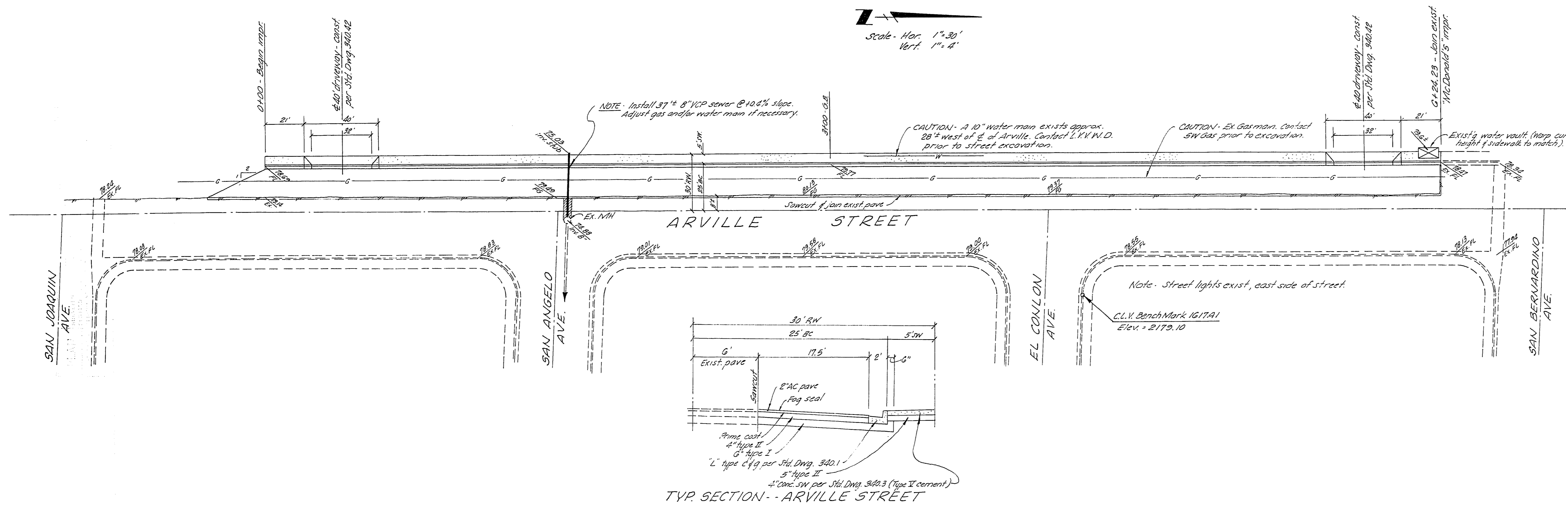
TYP. SECTION - ARVILLE STREET
