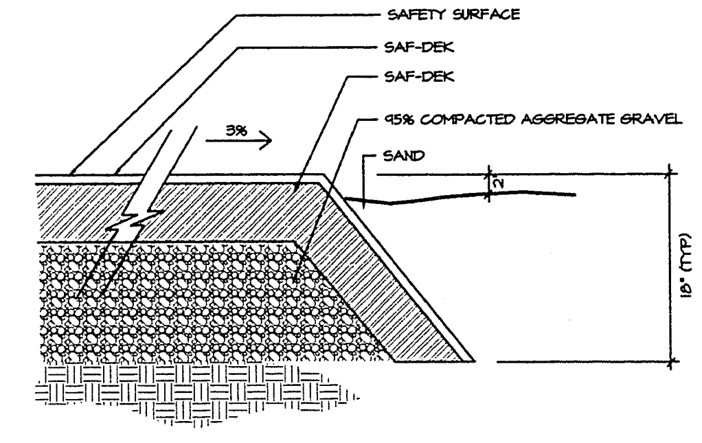
F SAF-DEK/SAND DETAIL
