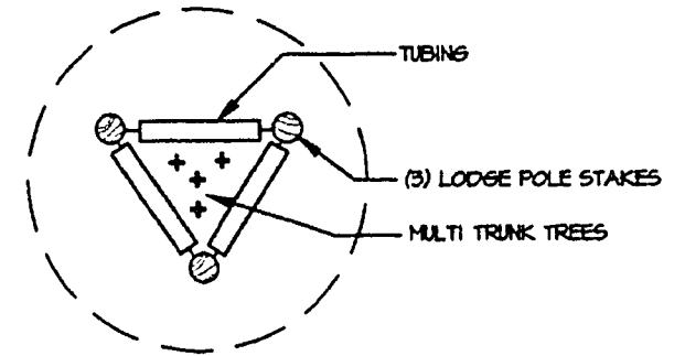
E MULTI TRUNK TREE STAKING
