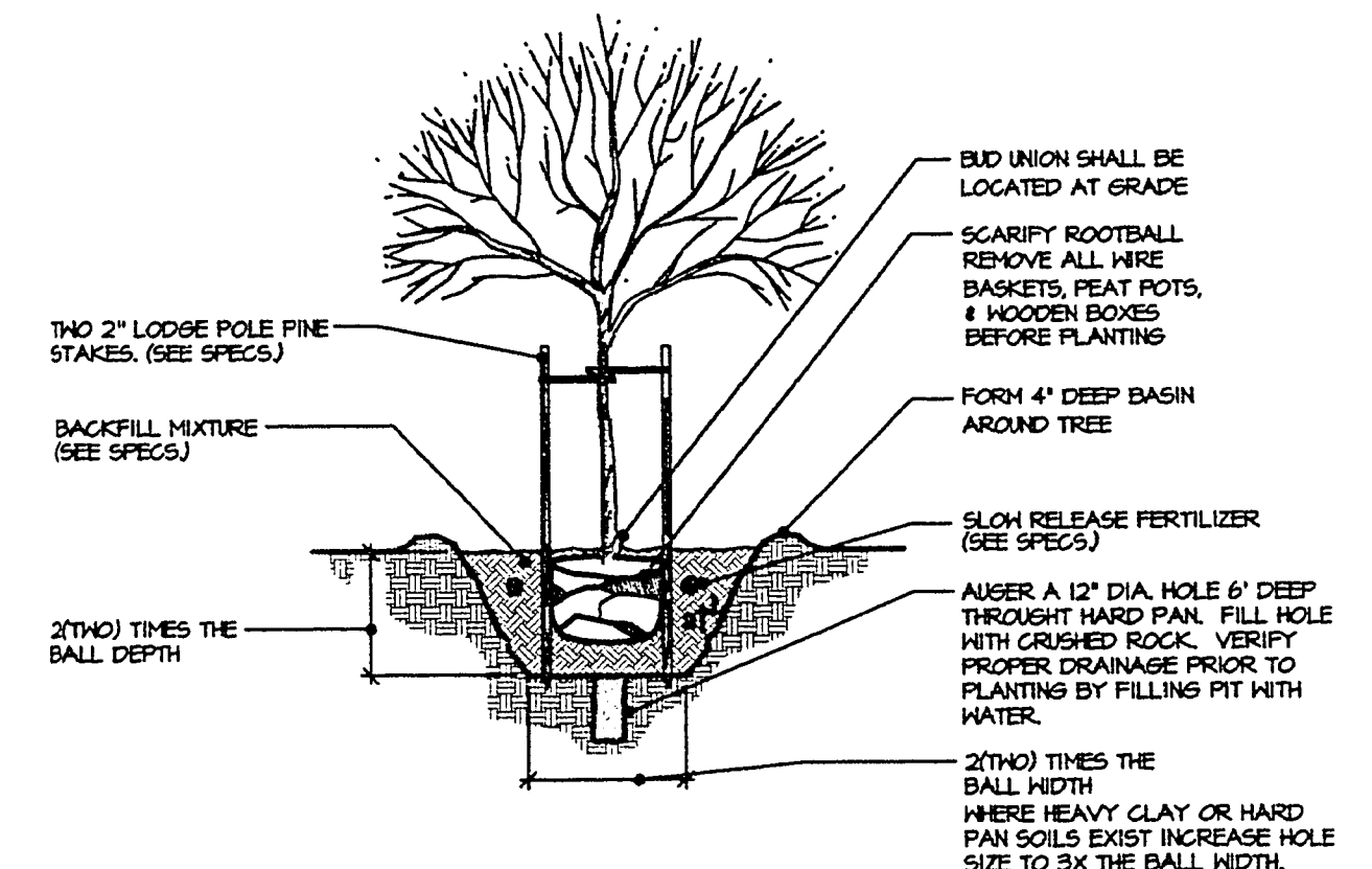
B TREE PLANTING AND STAKING
