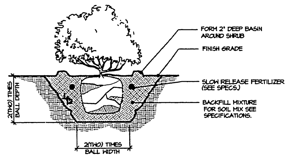
C SHRUB PLANTING
