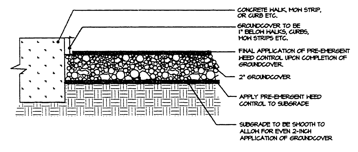
D GROUNDCOVER DETAIL
