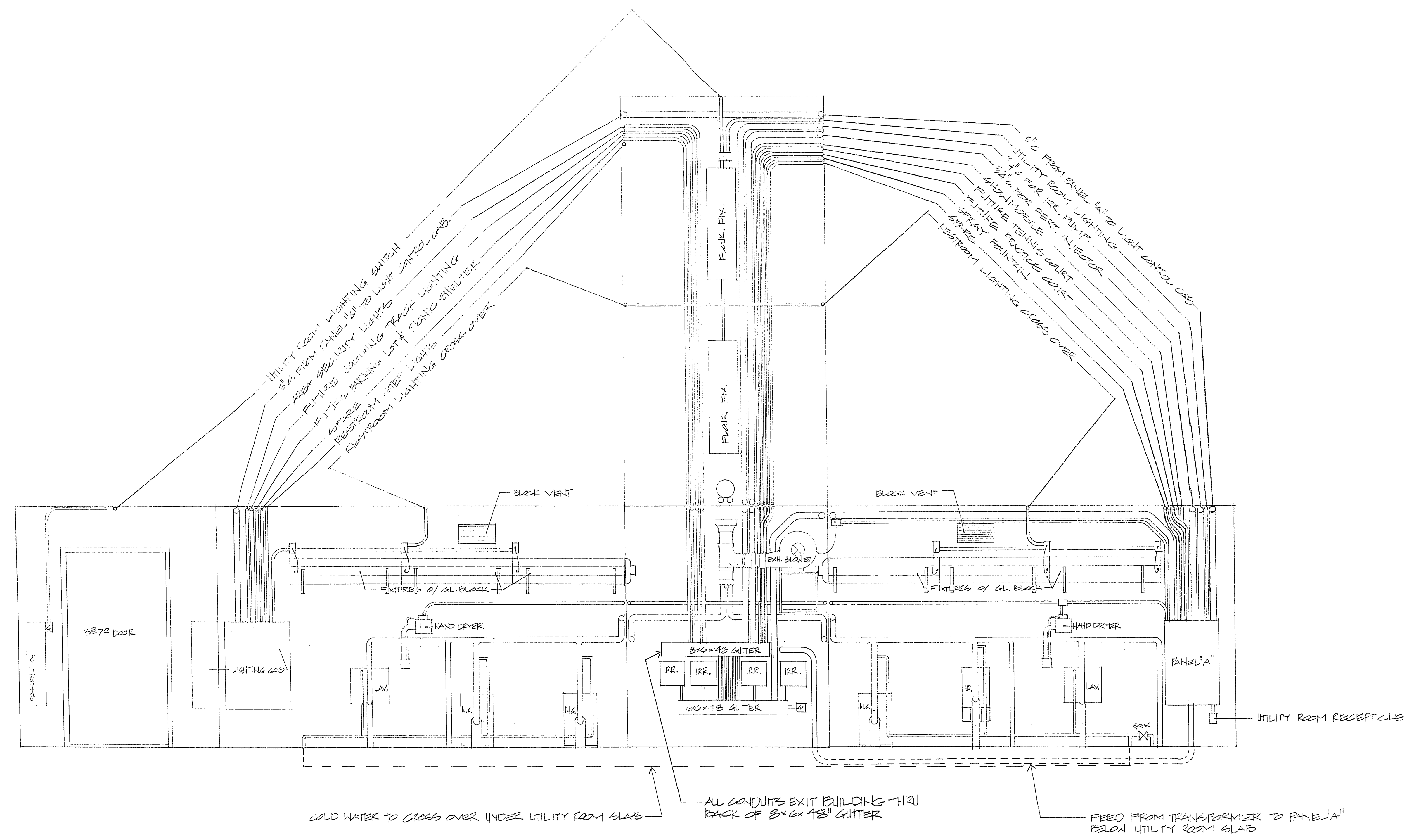
ANGEL PARK RESTROOM-UTILITY ROOM MECHANICAL/ELECTRICAL SCHEMATIC 1/8" = 1'-0"
