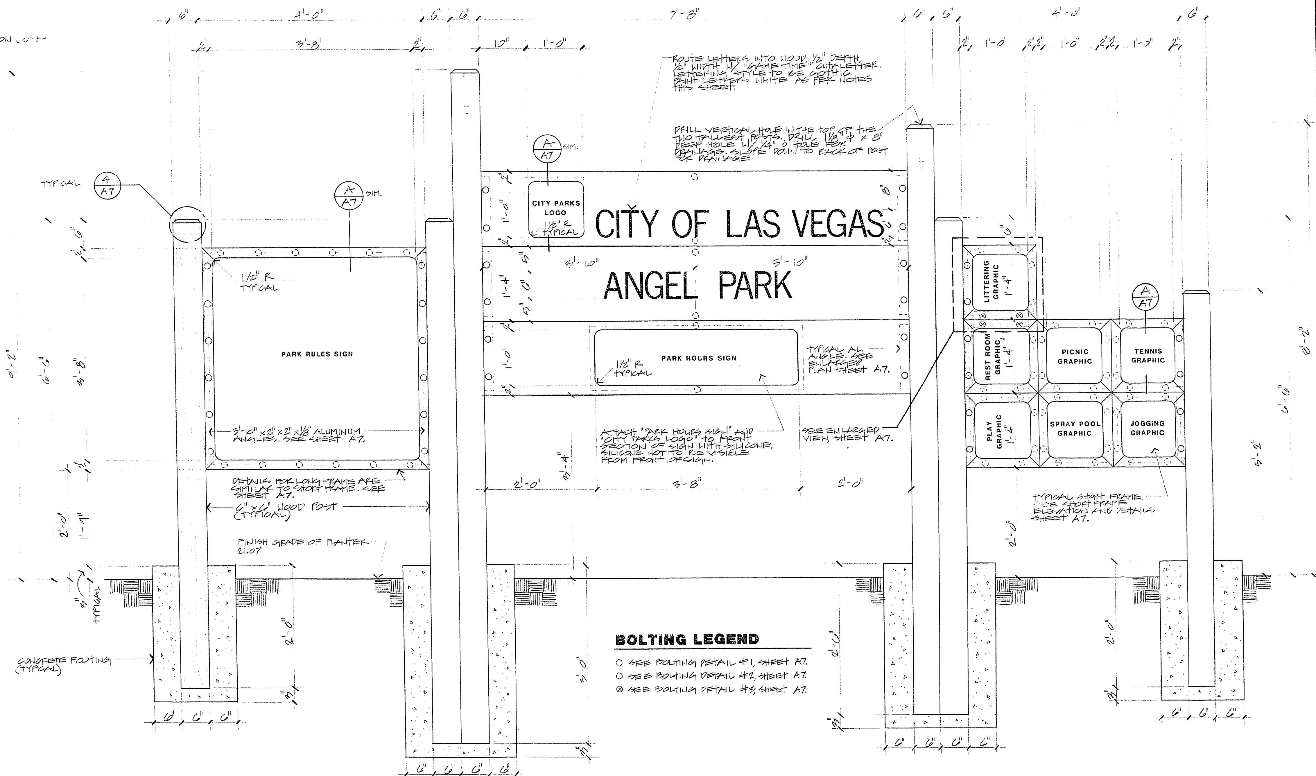
PARK SIGN ELEVATION - SECTION (FOLDED OUT)
