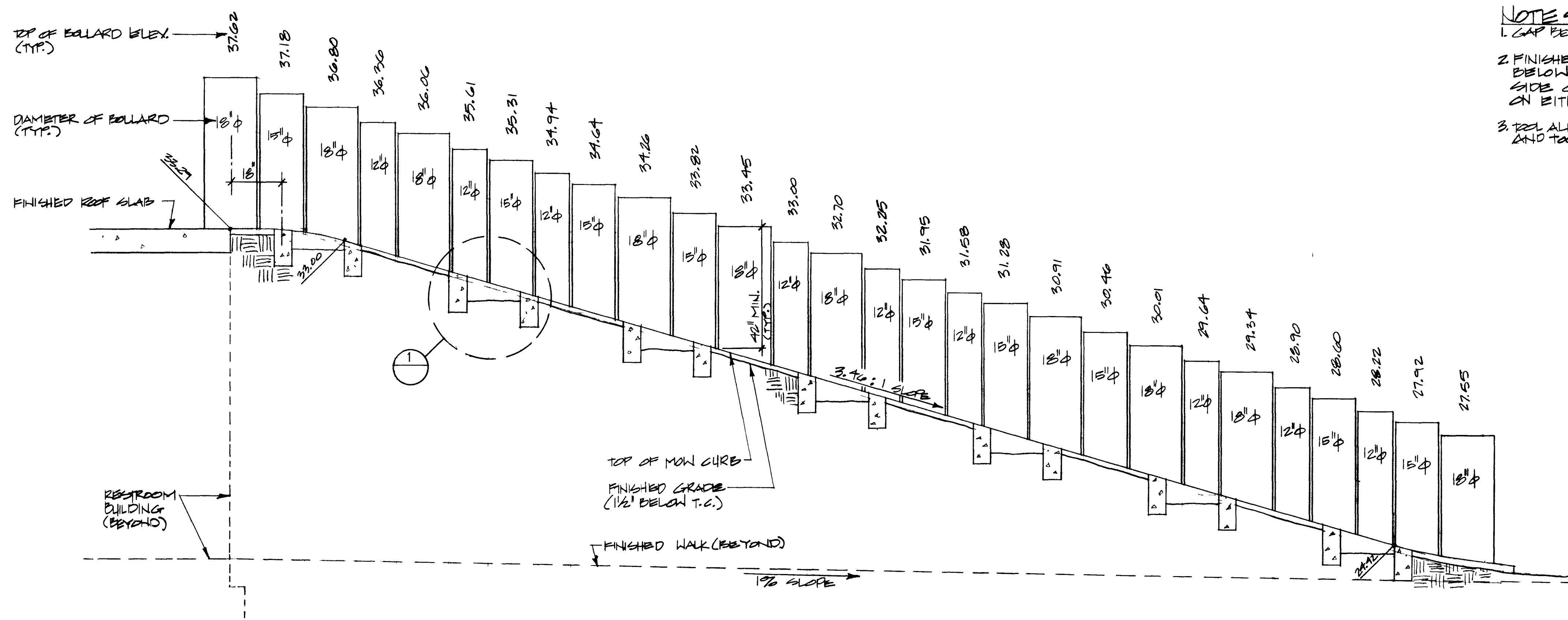
CROSS SECTION "B-B"
