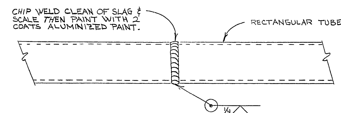
TYPICAL SUPPORT TUBE SPLICE
