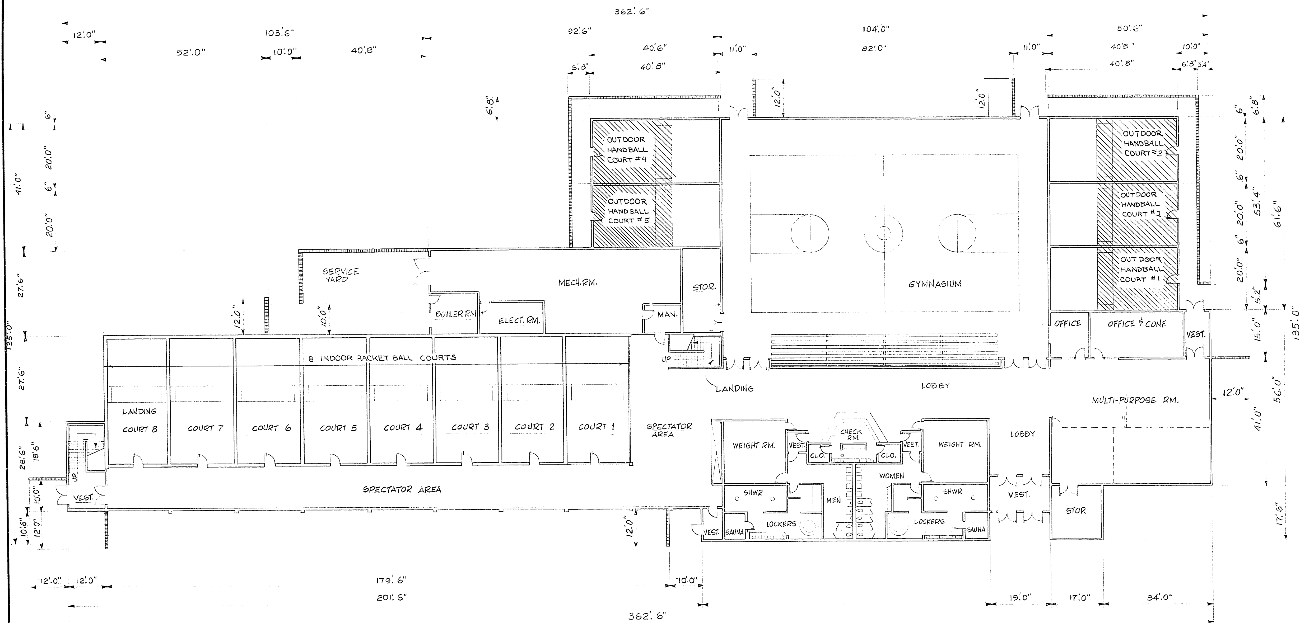
PLAN VIEW
