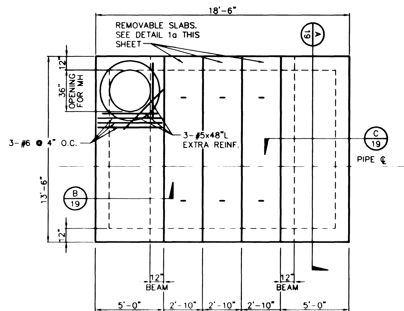
1 PLAN - ROOF SLAB SCALE: 1/4"=1'-0"
