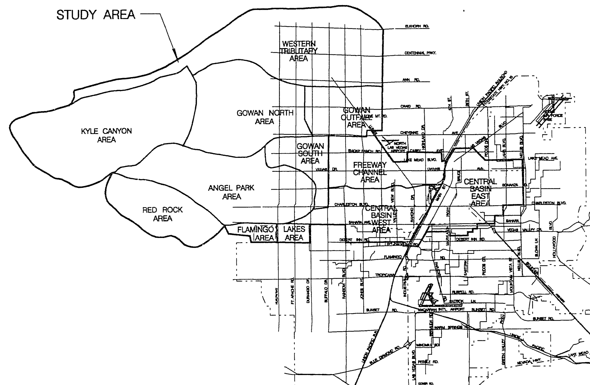
HYDROLOGIC MODELS
